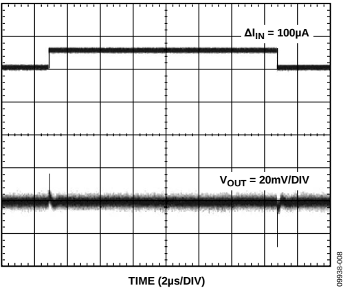
Figure 8. Output Response to a 100µA Input Current Change
