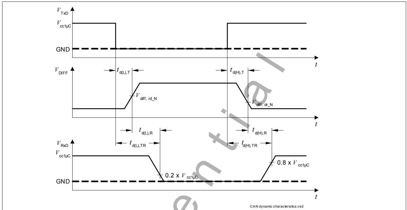
Figure 15 Timing Diagrams for Dynamic Characteristics
