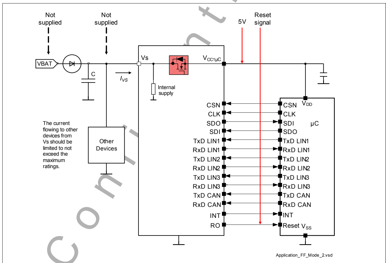
Figure 45 Application Hint for Factor Flash Mode
