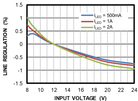
Line Regulation
