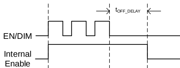
Figure 2: EN/DIM Timing Sequence
