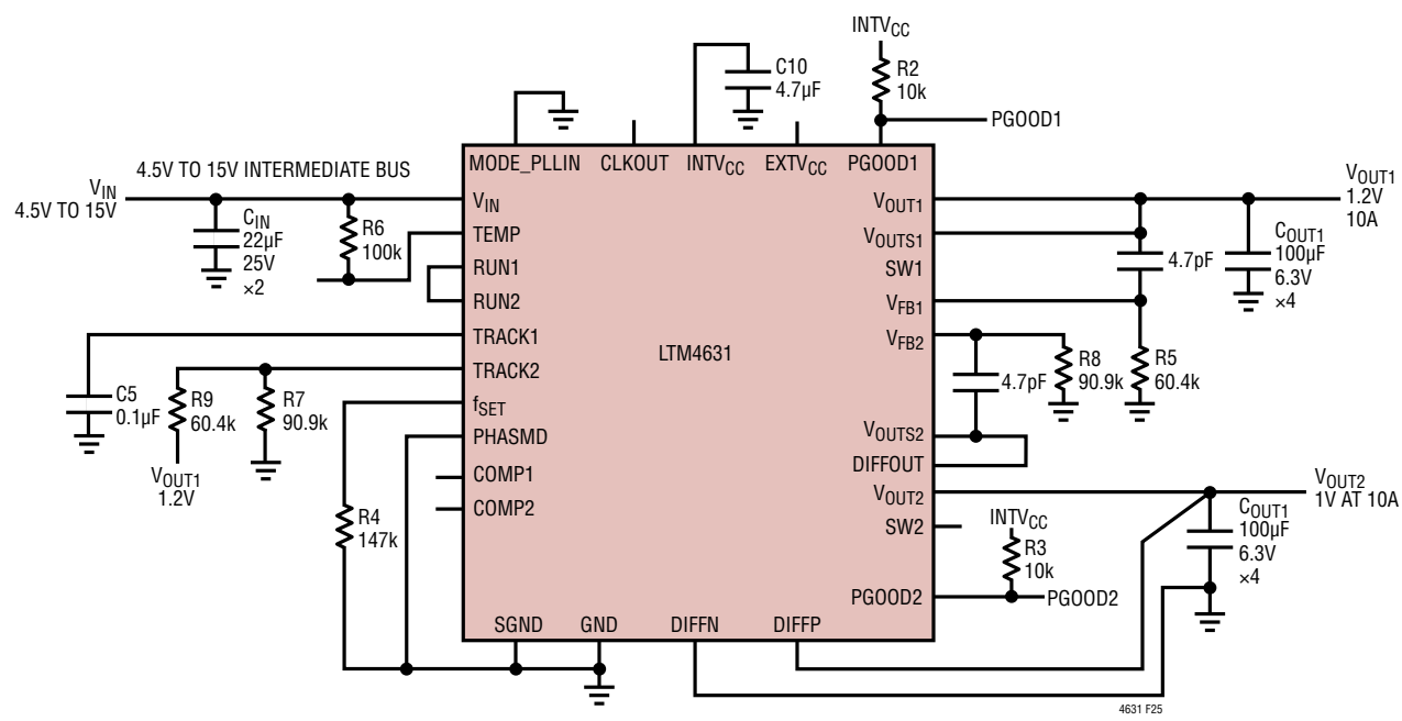
Figure 25. LTM4631 1.2V and 1V Output with Tracking Function
