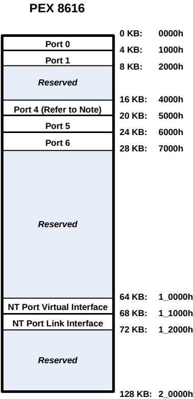
Figure 14-1. NT Mode Configuration Register Mapping to Memory-Mapped BAR
