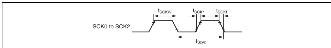
Figure 25.26 SCK Clock Input Timing
