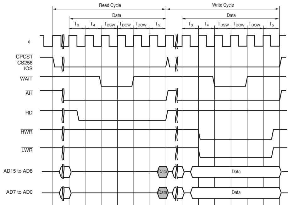
Figure 6.26 Example of Wait State Insertion Timing
