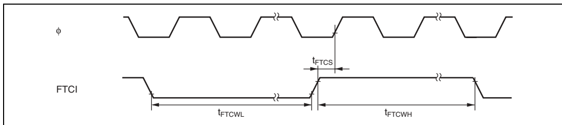
Figure 25.21 FRT Clock Input Timing
