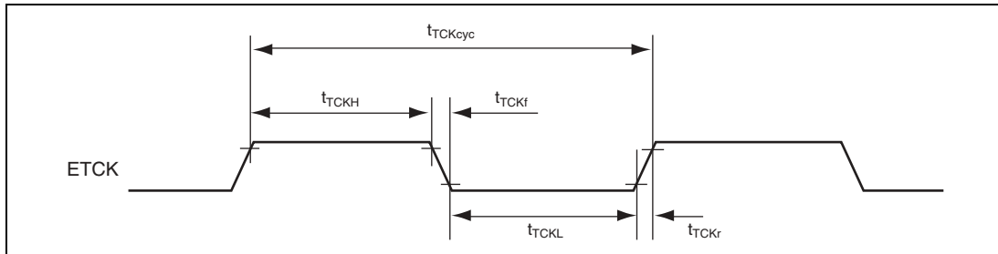
Figure 25.32 JTAG ETCK Timing
