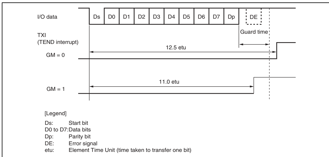
Figure 14.30 TEND Flag Set Timings during Transmission
