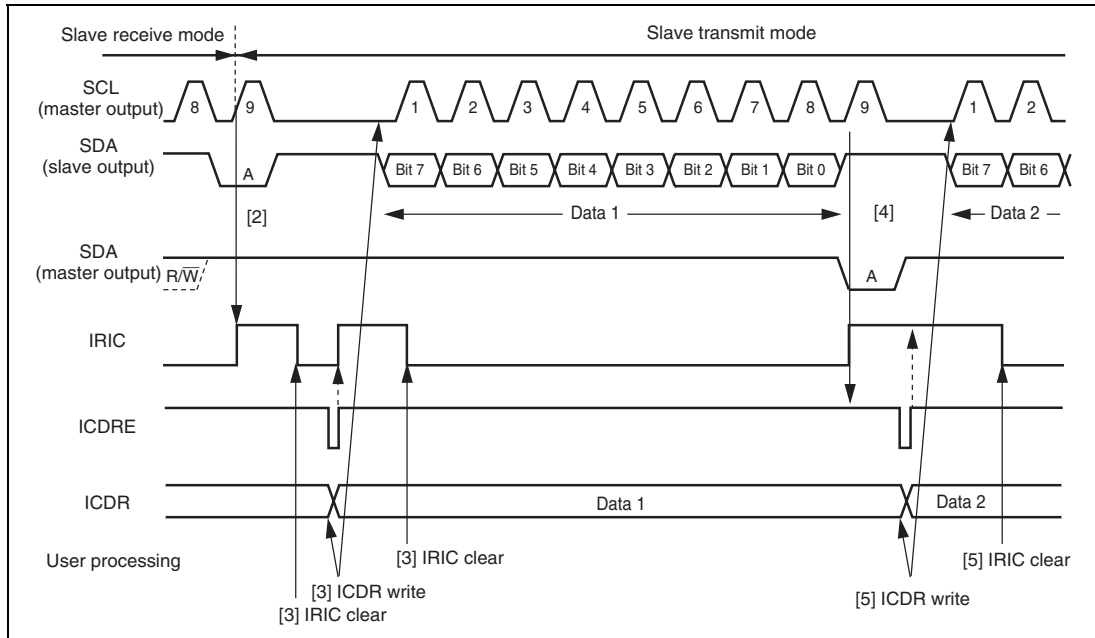
Figure 15.24 Slave Transmit Mode Operation Timing Example (MLS = 0)
