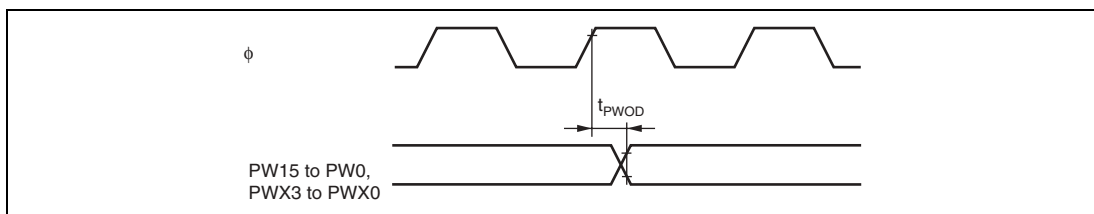
Figure 25.25 PWM, PWMX Output Timing
