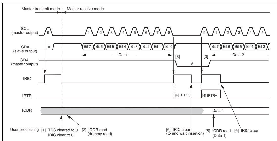
Figure 15.15 Master Receive Mode Operation Timing Example (MLS = ACKB = 0, WAIT = 1)
