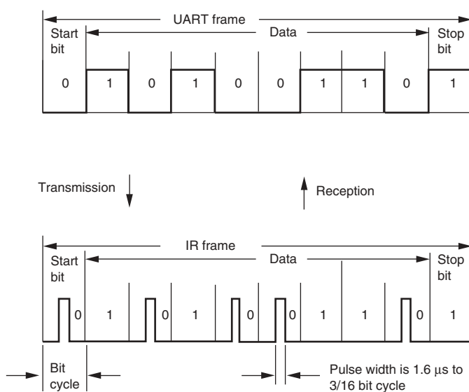
Figure 14.37 IrDA Transmission and Reception
