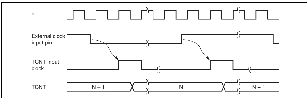
Figure 12.5 Count Timing for External Clock Input
