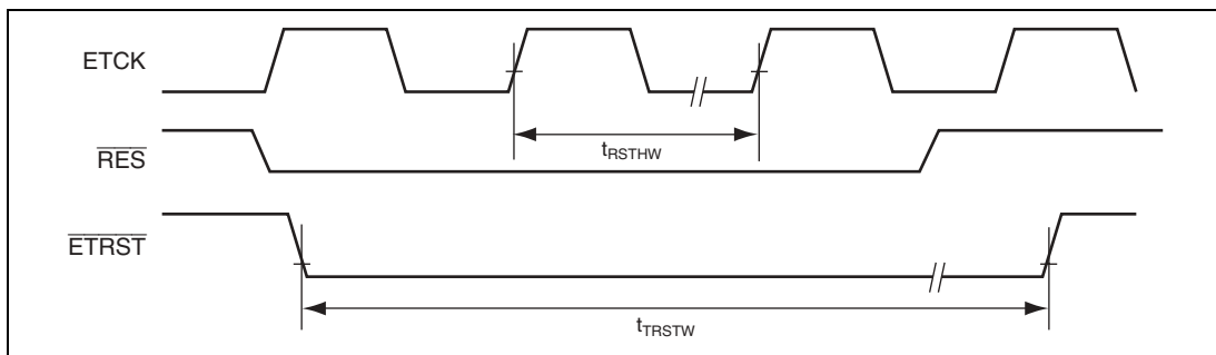
Figure 25.33 Reset Hold Timing
