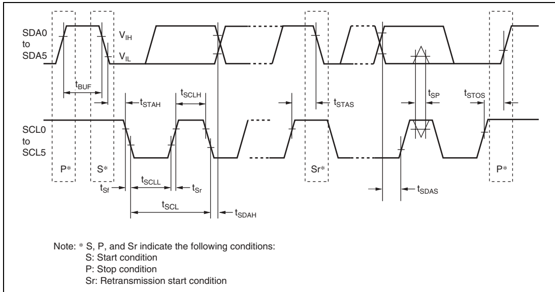
Figure 25.30 I²C Bus Interface Input/Output Timing
