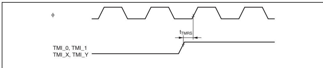
Figure 25.24 8-Bit Timer Reset Input Timing
