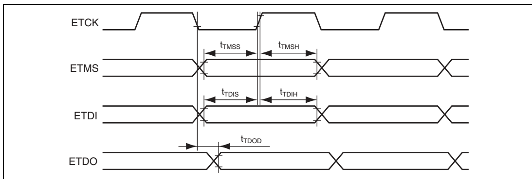
Figure 25.34 JTAG Input/Output Timing
