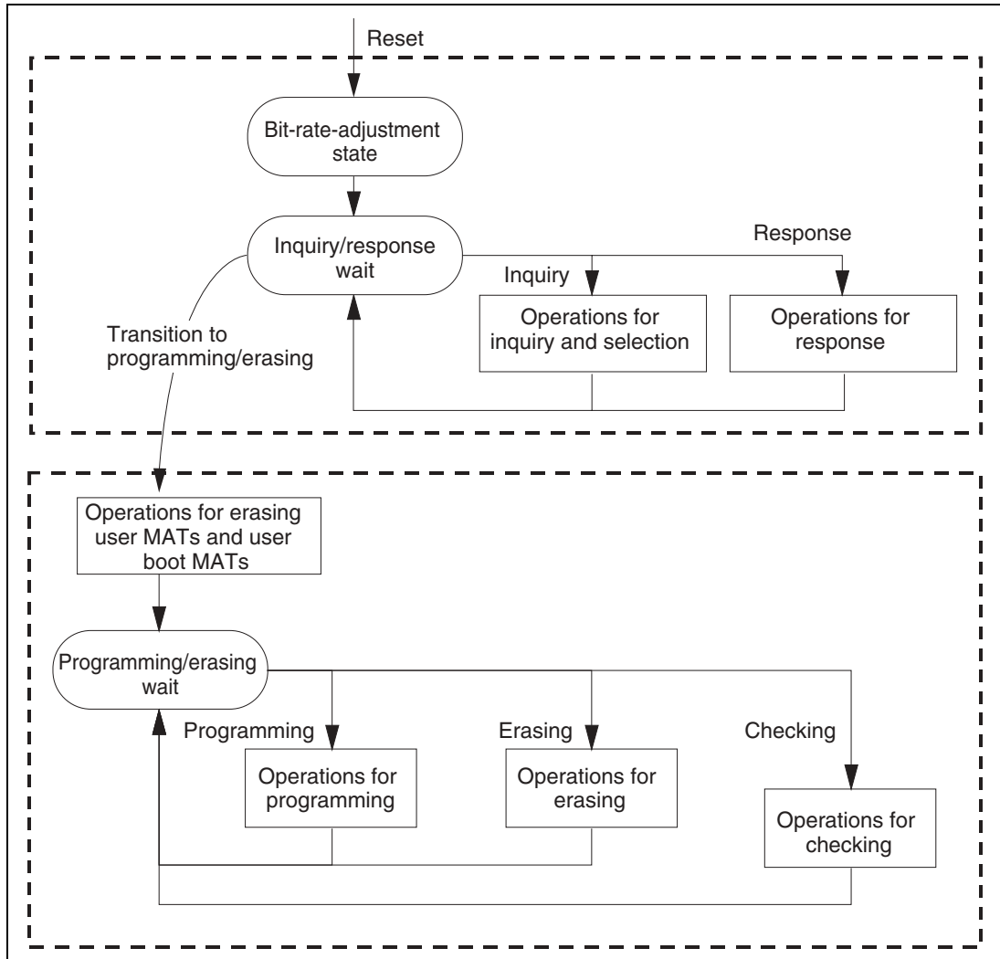
Figure 20.19 Boot Program States
