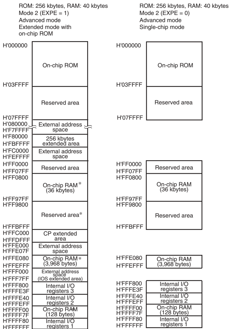
Figure 3.1 H8S/2168 Address Map
