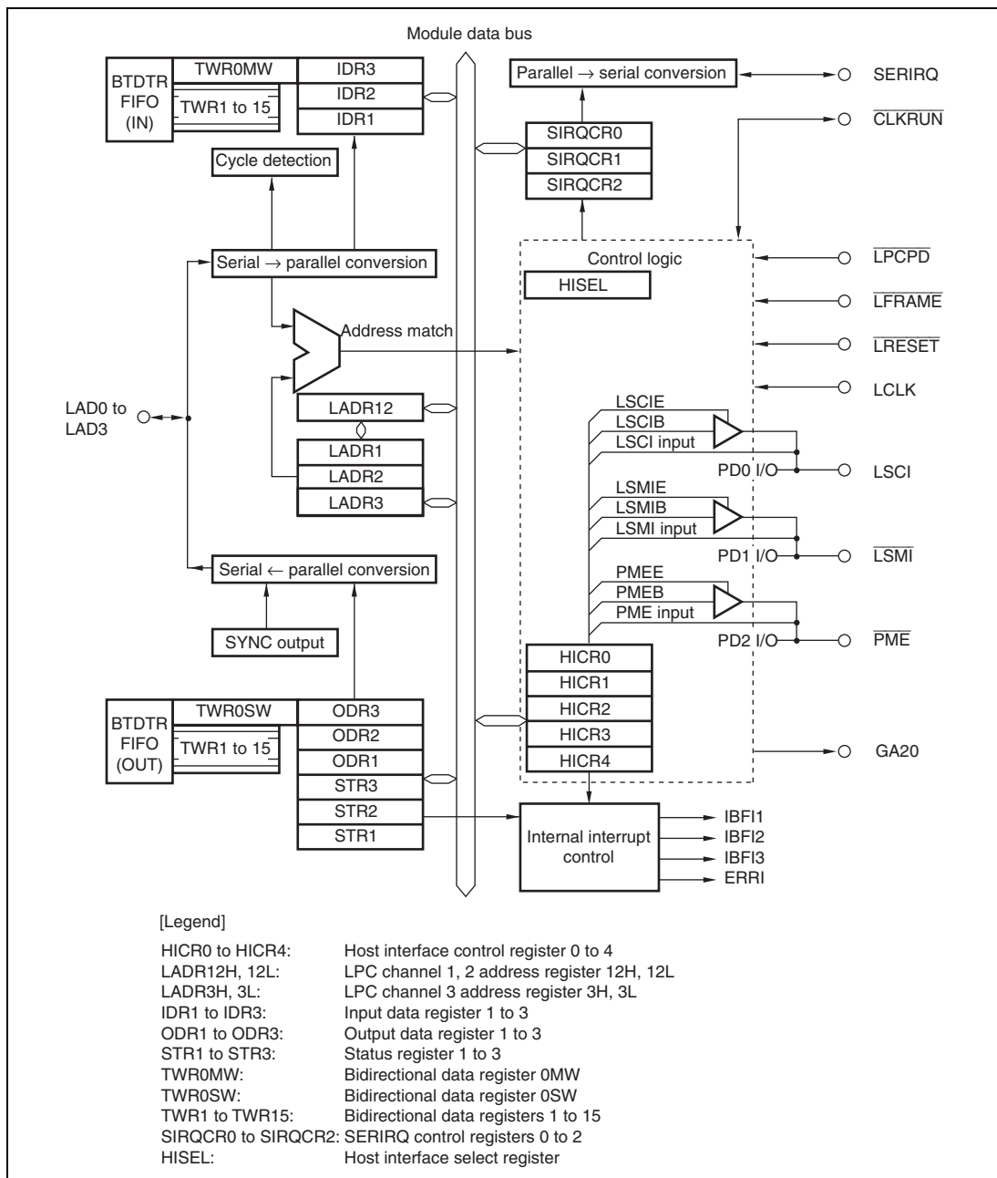
Figure 16.1 Block Diagram of LPC
