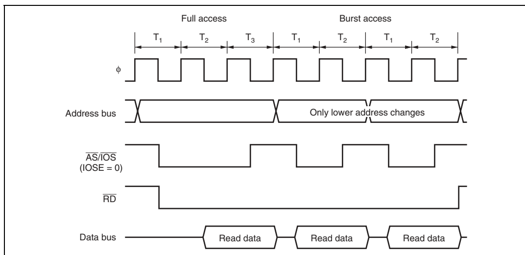
Figure 6.27 Access Timing Example in Burst ROM Space (AST = BRSTS1 = 1)
