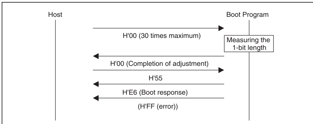
Figure 20.20 Bit-Rate-Adjustment Sequence
