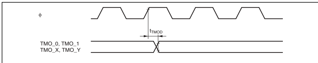
Figure 25.22 8-Bit Timer Output Timing
