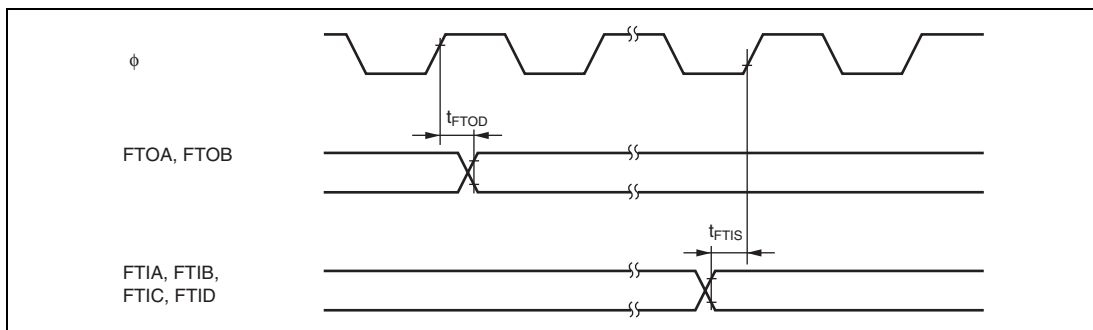
Figure 25.20 FRT Input/Output Timing
