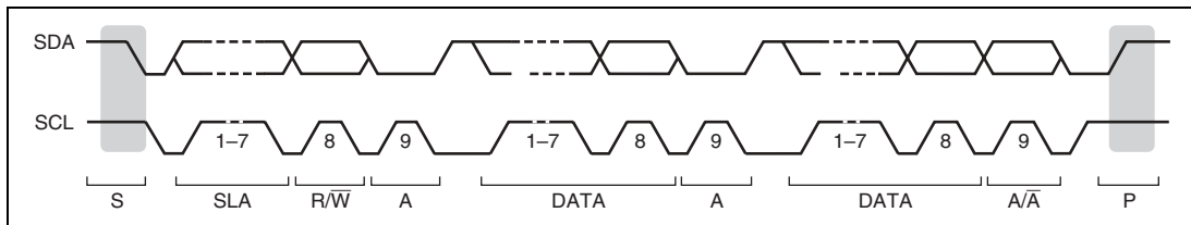
Figure 15.5 I²C Bus Timing
