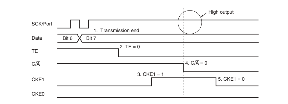
Figure 14.44 Prevention of Low Pulse Output at Switching from SCK Pins to Port Pins
