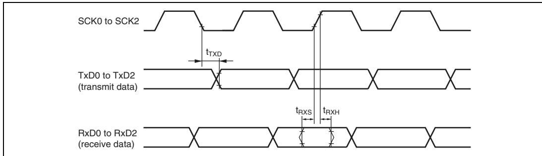
Figure 25.27 SCI Input/Output Timing (Clock Synchronous Mode)
