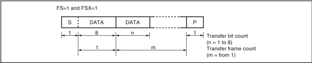
Figure 15.4 I 2 C Bus Data Formats (Serial Formats)
