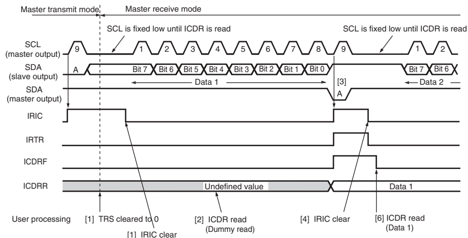
Figure 15.11 Master Receive Mode Operation Timing Example (MLS = WAIT = 0, HNDS = 1)
