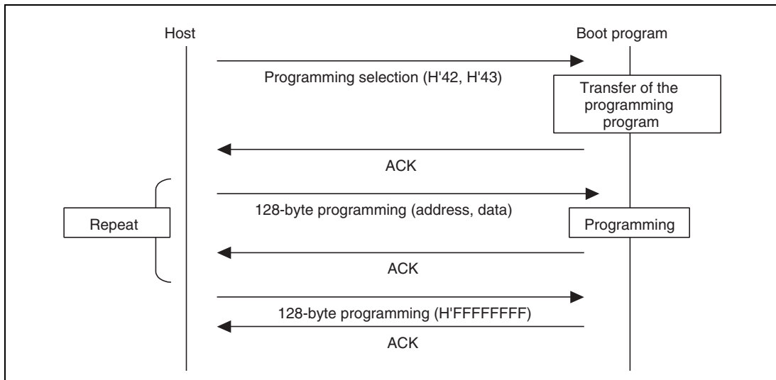
Figure 20.23 Programming Sequence
