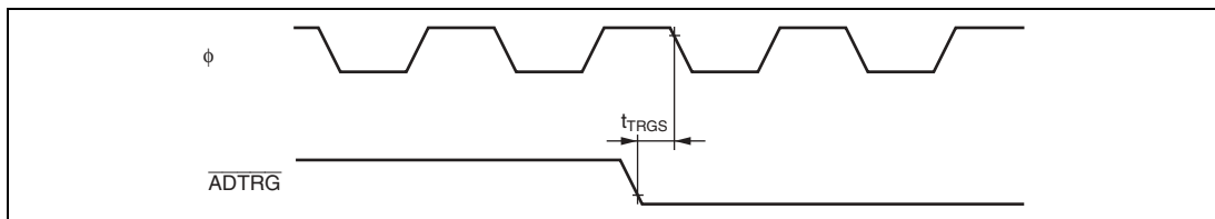
Figure 25.28 A/D Converter External Trigger Input Timing
