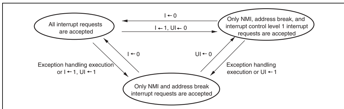
Figure 5.6 State Transition in Interrupt Control Mode 1
