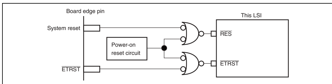
Figure 21.3 Reset Signal Circuit Without Reset Signal Interference
