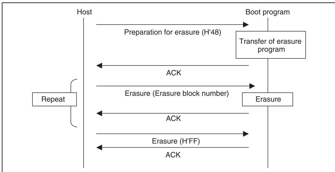
Figure 20.24 Erasure Sequence
