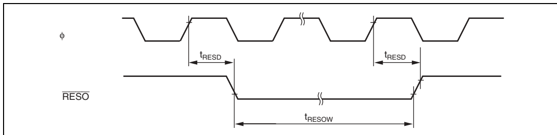
Figure 25.29 WDT Output Timing ( \overline{RESO} )
