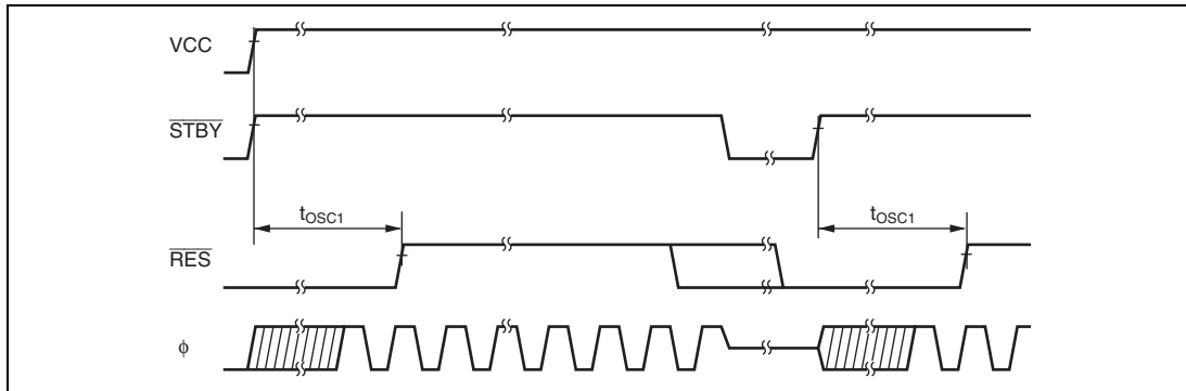
Figure 25.5 Oscillation Stabilization Timing
