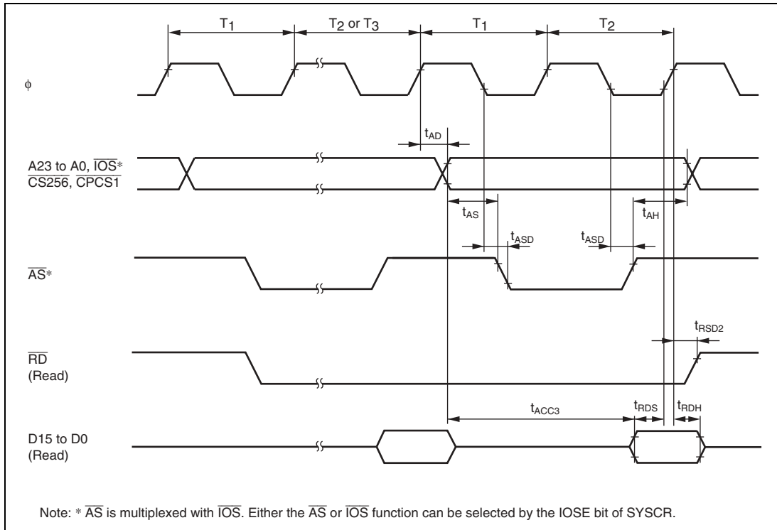
Figure 25.15 Burst ROM Access Timing/2-State Access
