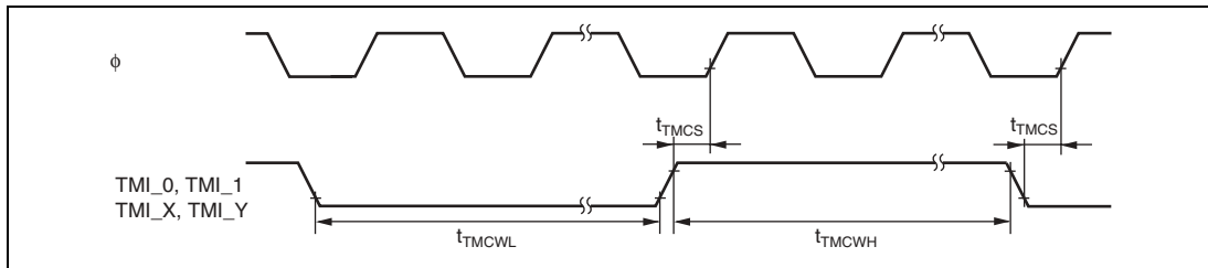
Figure 25.23 8-Bit Timer Clock Input Timing
