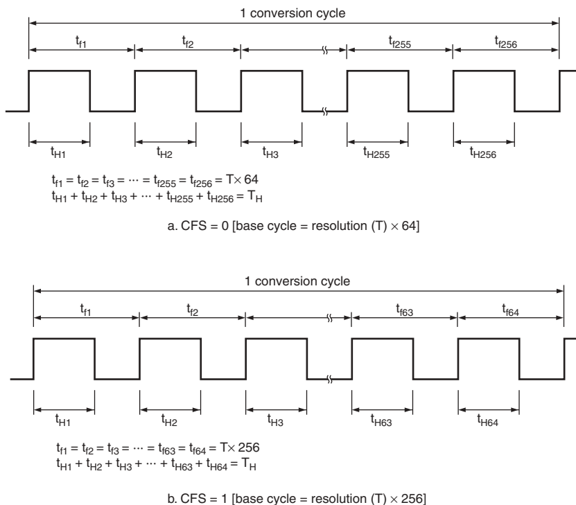
Figure 10.4 Output Waveform (OS = 1, DADR corresponds to T_H )
