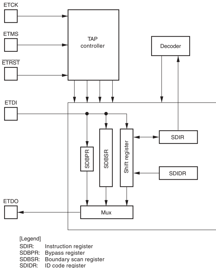
Figure 21.1 JTAG Block Diagram
