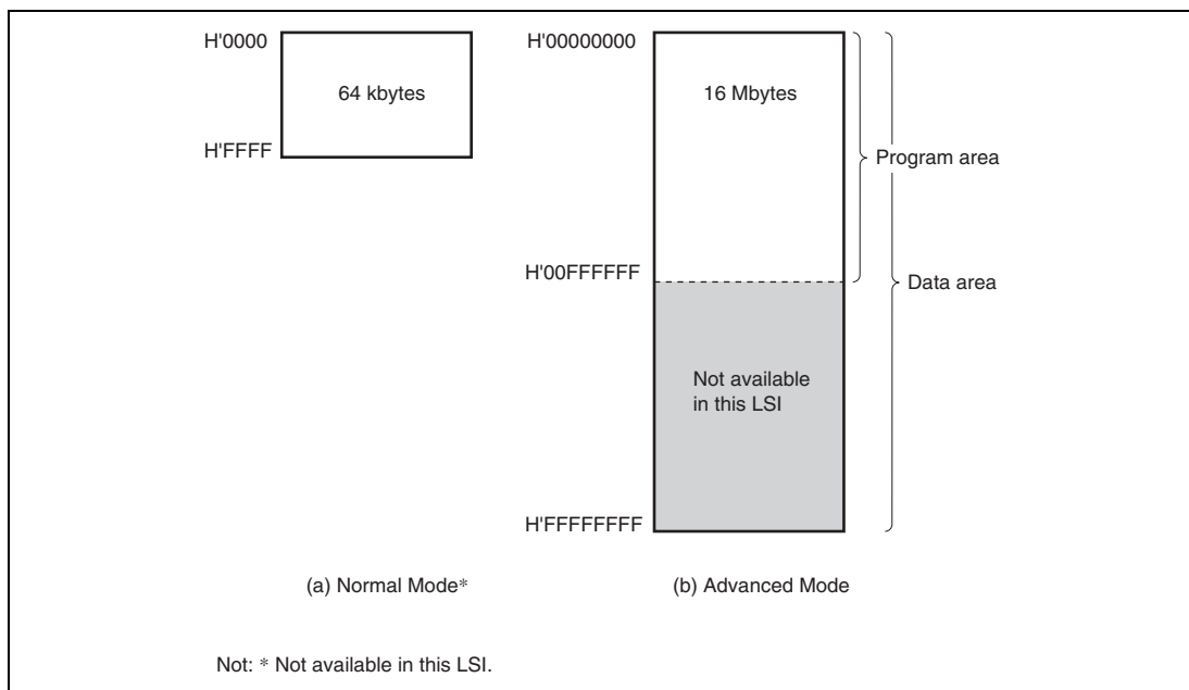
Figure 2.5 Memory Map
