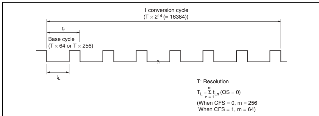
Figure 10.2 PWMX (D/A) Operation
