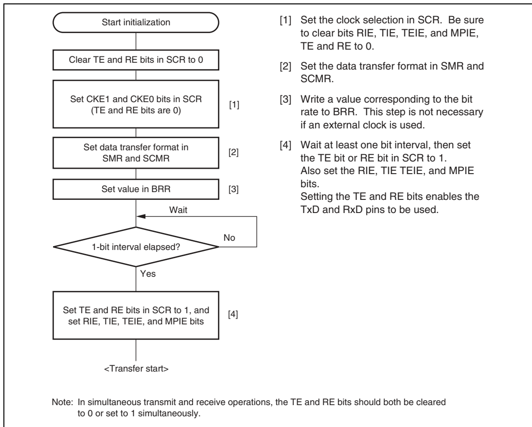
Figure 14.18 Sample SCI Initialization Flowchart
