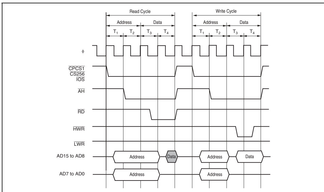
Figure 6.17 Bus Timing for 16-Bit, 2-State Access Space (2) (Even Byte Access)
