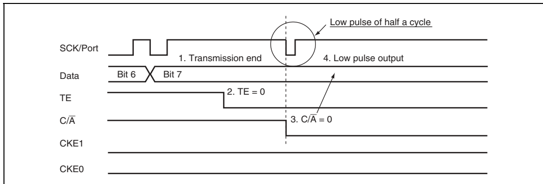
Figure 14.43 Switching from SCK Pins to Port Pins
