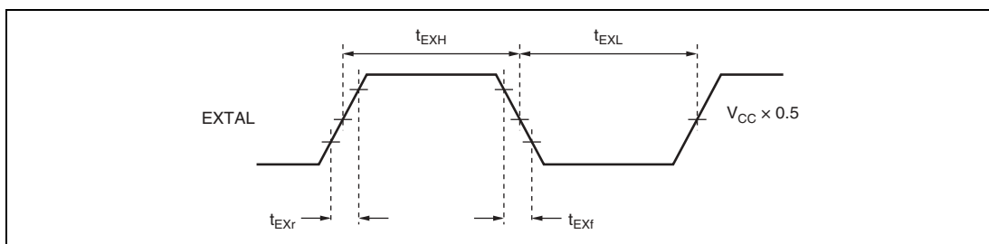
Figure 25.7 External Clock Input Timing
