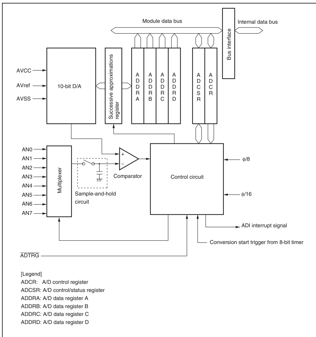
Figure 18.1 Block Diagram of A/D Converter
