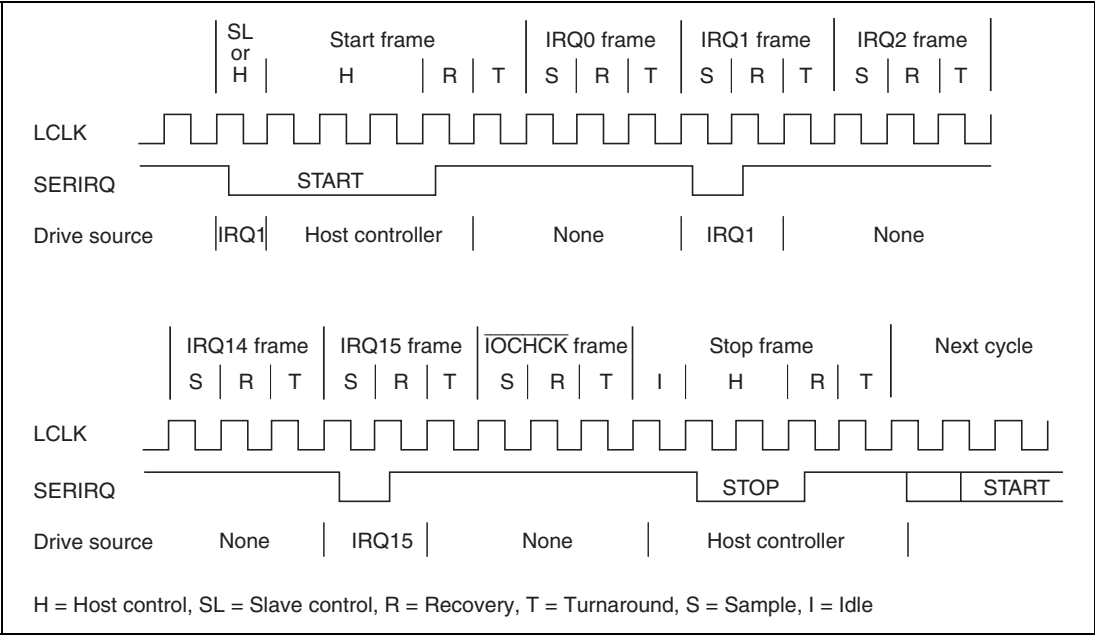
Figure 16.10 SERIRQ Timing
