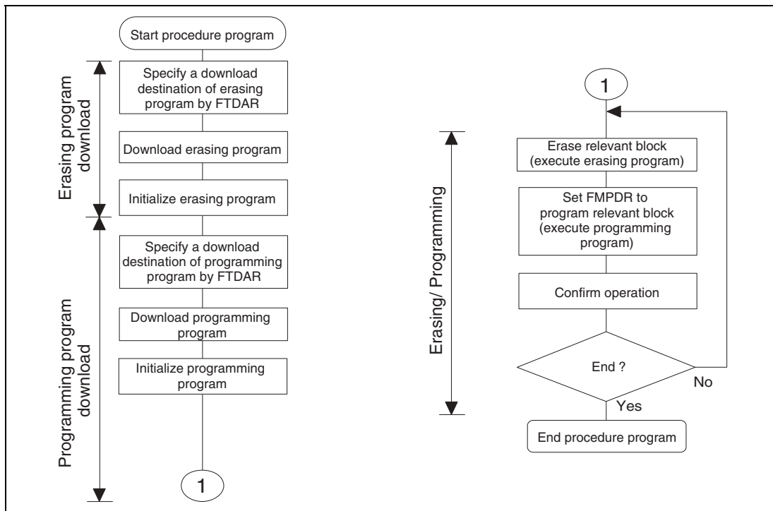
Figure 20.13 Repeating Procedure of Erasing and Programming
