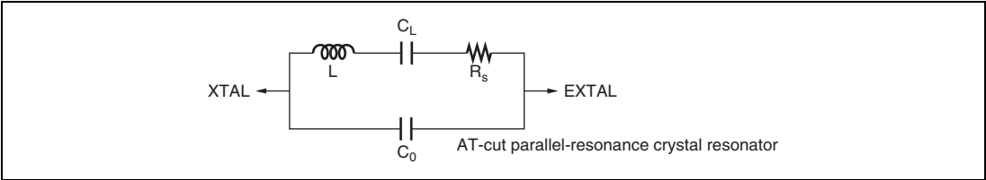
Figure 22.3 Equivalent Circuit of Crystal Resonator
