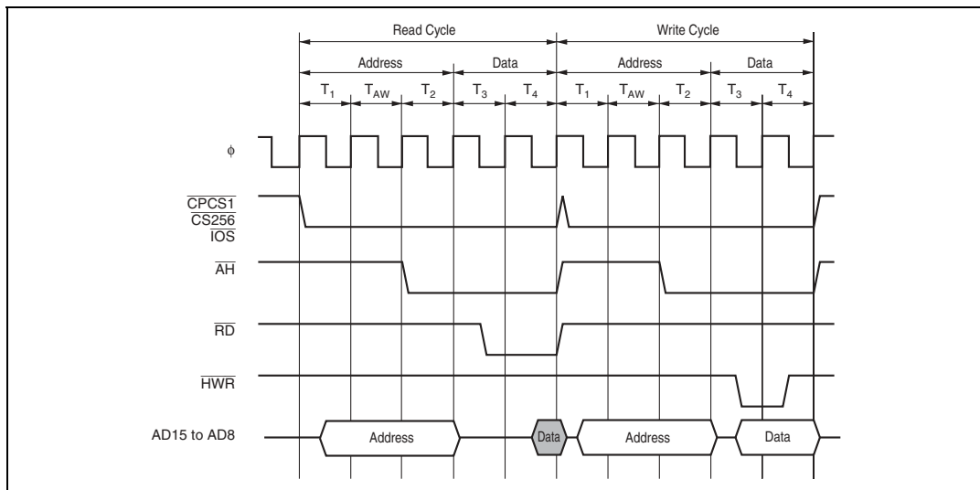
Figure 6.13 Bus Timing for 8-Bit, 2-State Access Space
