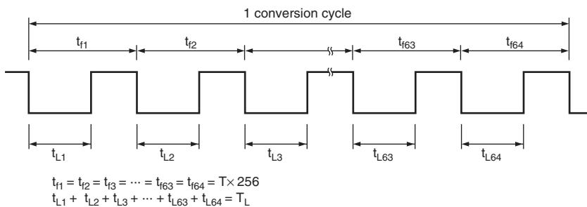
Figure 10.3 Output Waveform (OS = 0, DADR corresponds to T_L )
