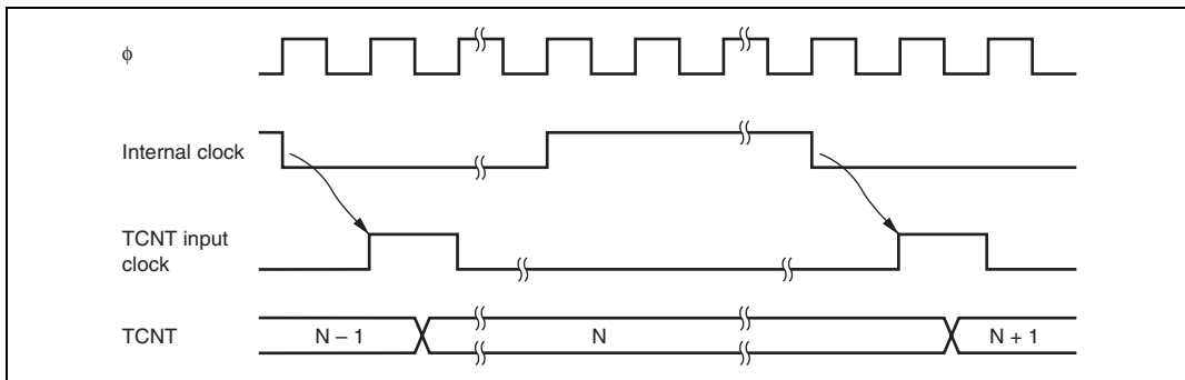
Figure 12.4 Count Timing for Internal Clock Input
