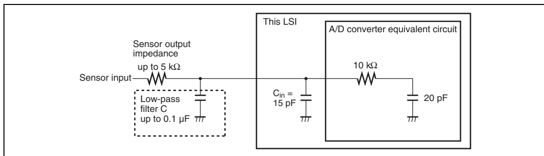
Figure 18.6 Example of Analog Input Circuit
