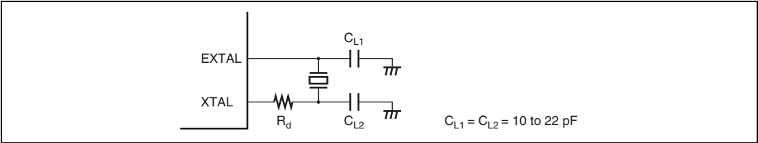
Figure 22.2 Typical Connection to Crystal Resonator
