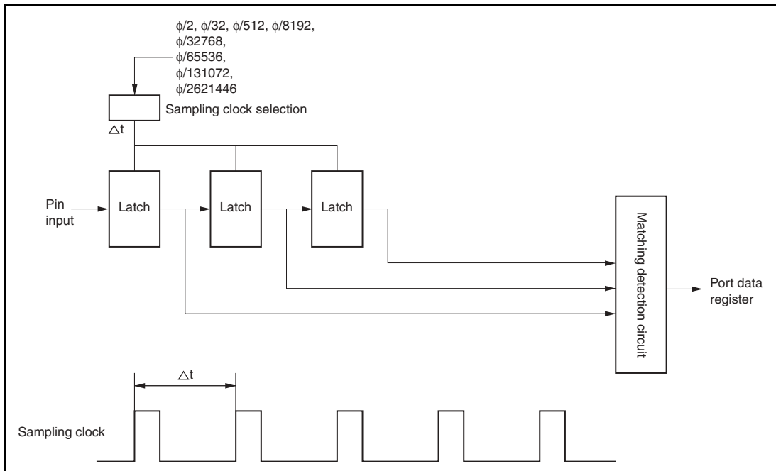
Figure 8.1 Noise Canceler Circuit
