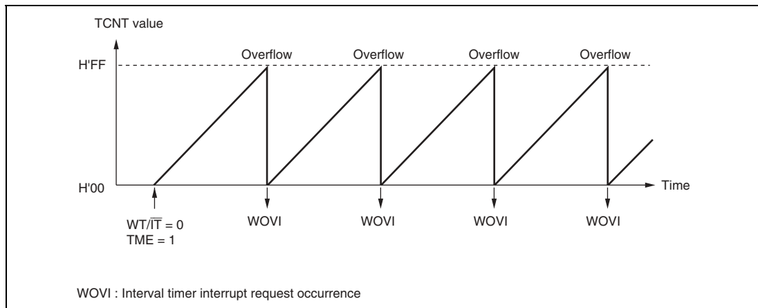
Figure 13.3 Interval Timer Mode Operation
