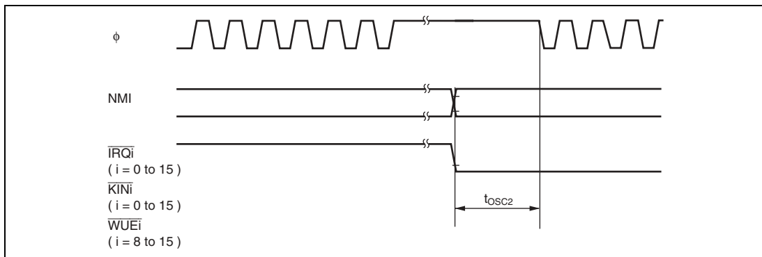
Figure 25.6 Oscillation Stabilization Timing (Exiting Software Standby Mode)
