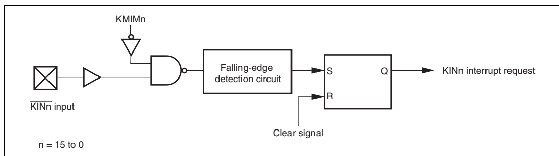
Figure 5.3 Block Diagram of Interrupts KIN15 to KIN0 and WUE15 to WUE8 (Example of KIN15 to KIN0)
