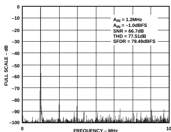
Figure 8. FFT Plot
