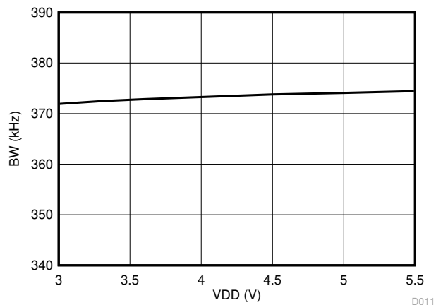
Figure 6-11. Output Bandwidth vs Supply Voltage
