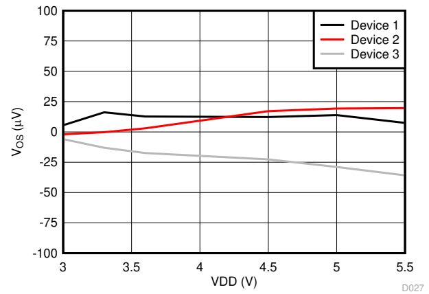
Figure 6-18. Offset Error vs Supply Voltage
