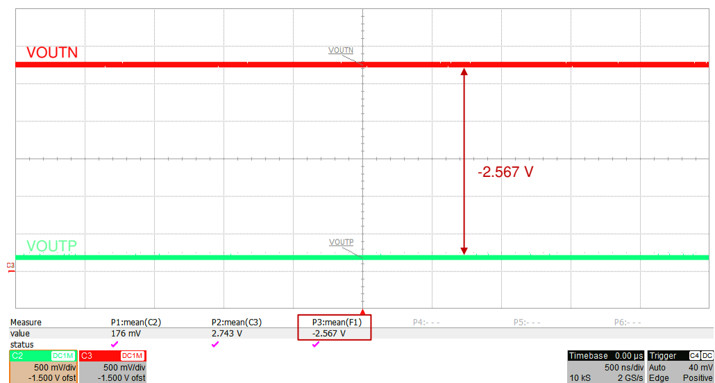
Figure 7-5. Typical Fail-Safe Output of the AMC3330
