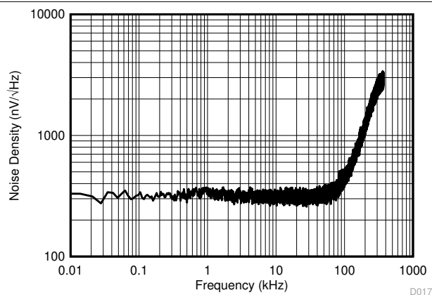
Figure 6-29. Input-Referred Noise Density vs Frequency
