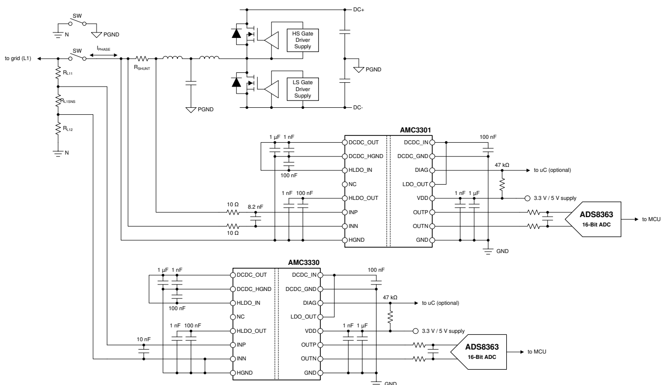
Figure 8-1. The AMC3330 in a Solar Inverter Application
