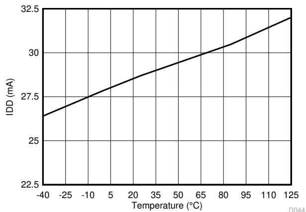
Figure 6-35. Input-Supply Current vs Temperature
