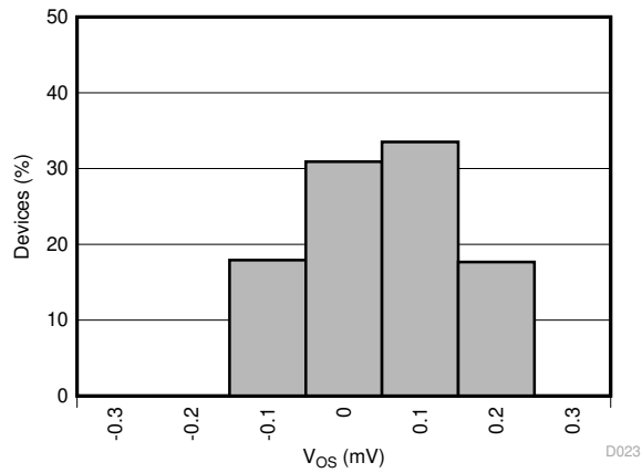
Figure 6-17. Offset Error Histogram
