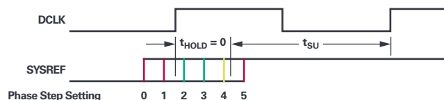
Figure 6. Programmable phase delay for SYSREF to meet timing.
