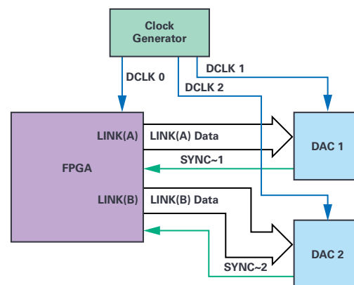
Figure 9. Subclass 2 multiple DAC application.
