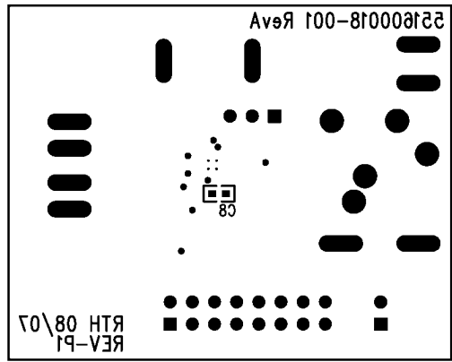
FIGURE 15. Bottom Silkscreen
