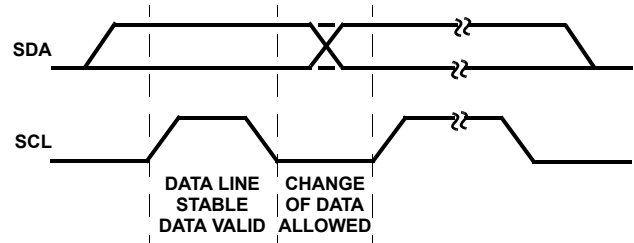
FIGURE 22. DATA VALIDITY
