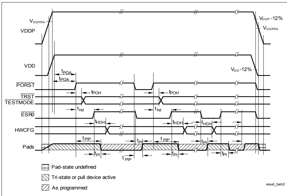
Figure 25 Power, Pad and Reset Timing
