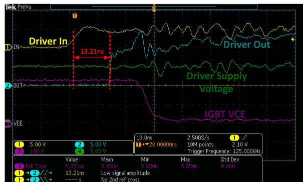
Figure 8-3. UCC27624 Used to Drive IGBT in the Boost Converter
