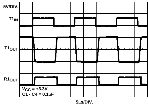
FIGURE 7. LOOPBACK TEST AT 120\text{Kbps}
