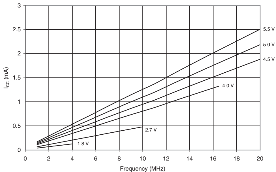
Figure 20-8. Idle Supply Current vs. V_{CC} (Internal Calibrated Oscillator, 8 MHz)
