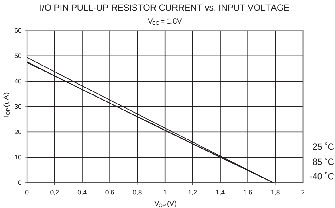
Figure 20-122. Pull-Up Resistor Current vs. Input Voltage (I/O Pin, V_{CC} = 1.8V )
