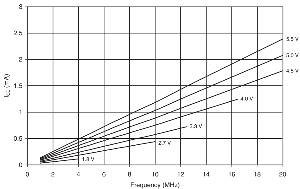
Figure 20-110. Idle Supply Current vs. V_{CC} (Internal Calibrated Oscillator, 8 MHz)
