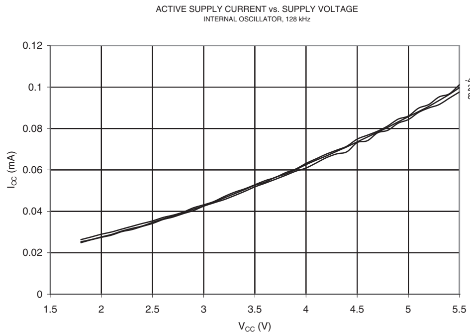
Figure 20-107. Active Supply Current vs. V_{CC} (Internal Calibrated Oscillator, 128 kHz)
