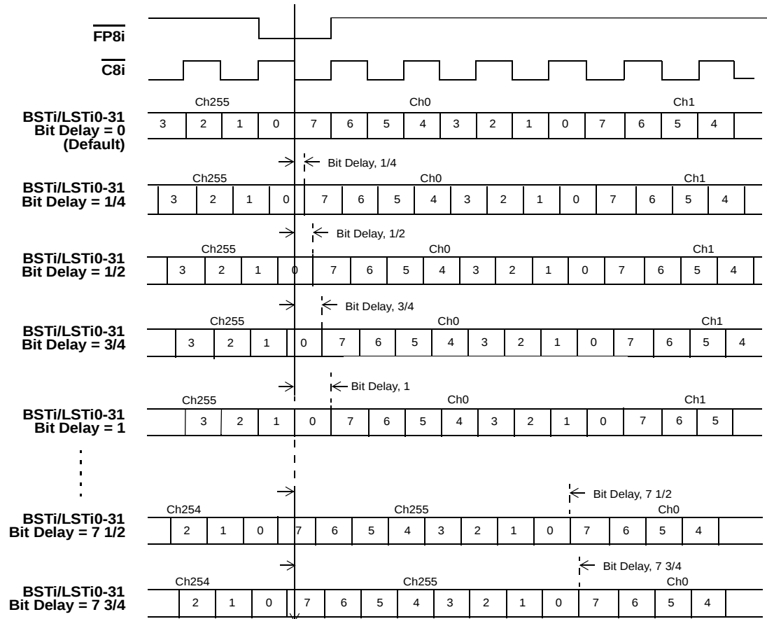
Figure 10 - Backplane and Local Input Bit Delay Timing Diagram for Data Rate of 16 Mbps
