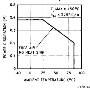
5-Lead Plastic SOT23 Maximum Power Dissipation vs Ambient Temperature
