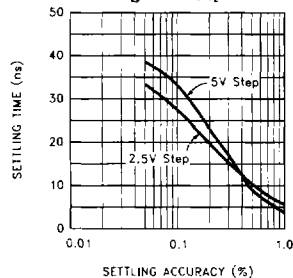
Settling Time vs Settling Accuracy
