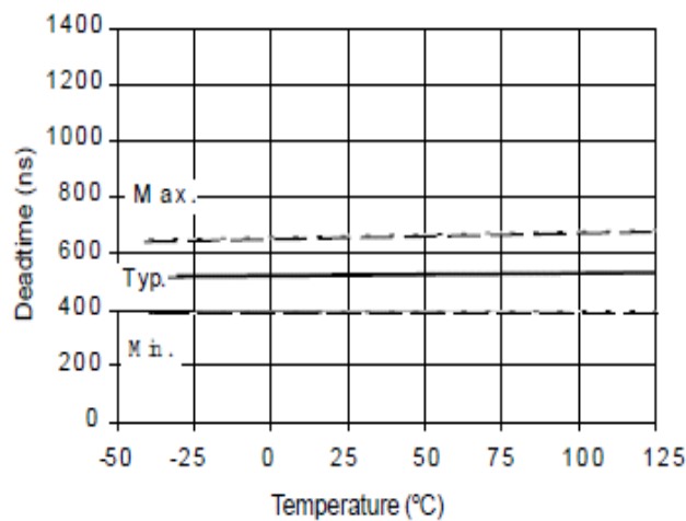
Figure 8A. Deadtime vs. Temperature
