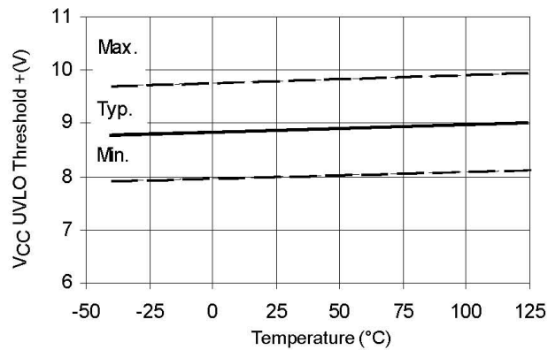
Figure 18A. V_{CC}UV_{BS} Undervoltage Threshold(+) vs. Temperature
