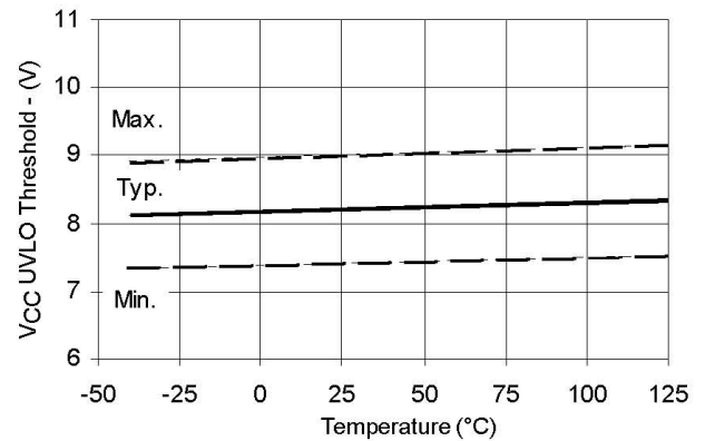
Figure 18B. V_{CC}UV_{BS} Undervoltage Threshold(-) vs. Temperature
