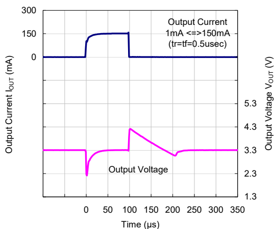
VR=3.3V, C_{OUT}=0.1\mu\text{F}
