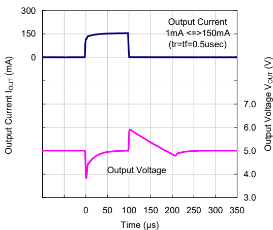
VR=5.0V, C_{OUT}=0.1\mu\text{F}
