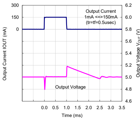
VR=5.0V, C_{OUT}=10\mu\text{F}
