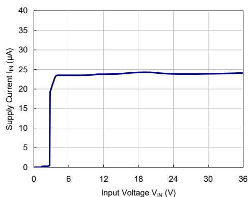
VR=5.0V
