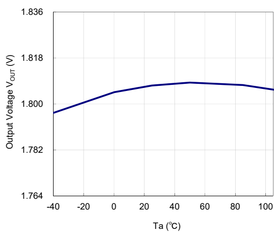
VR=1.8V
