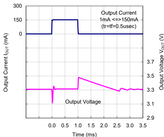
VR=3.3V, C_{OUT}=10\mu\text{F}
