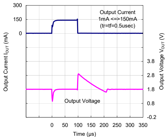
VR=1.8V, C_{OUT}=0.1\mu\text{F}
