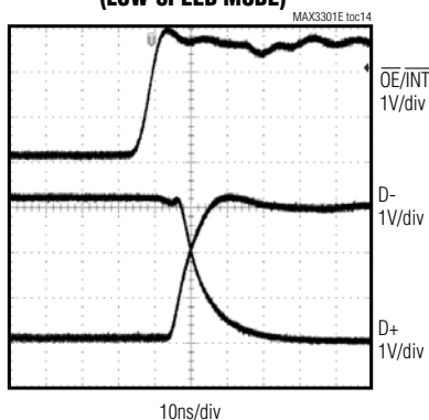
DRIVER DISABLE DELAY (LOW-SPEED MODE)
