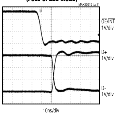
DRIVER ENABLE DELAY (FULL-SPEED MODE)
