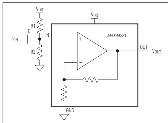
Figure 1. How to Use the MAX44281 in AC-Coupled Applications
