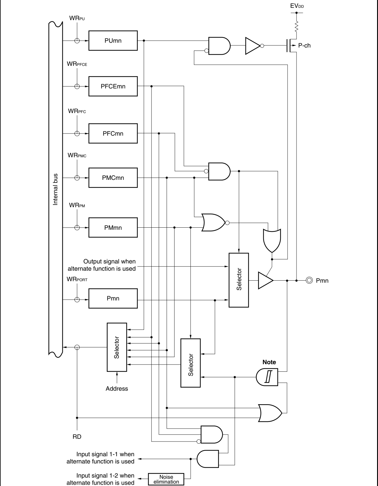
Figure 4-20. Block Diagram of Type U-4
