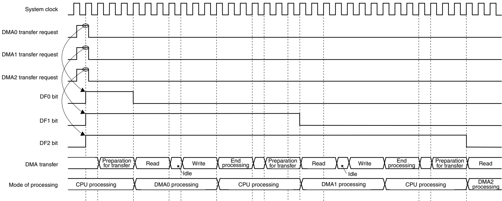
Figure 15-1. Priority of DMA (1)
