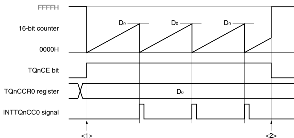
Figure 8-12. Flow of Software Processing in External Event Count Mode
