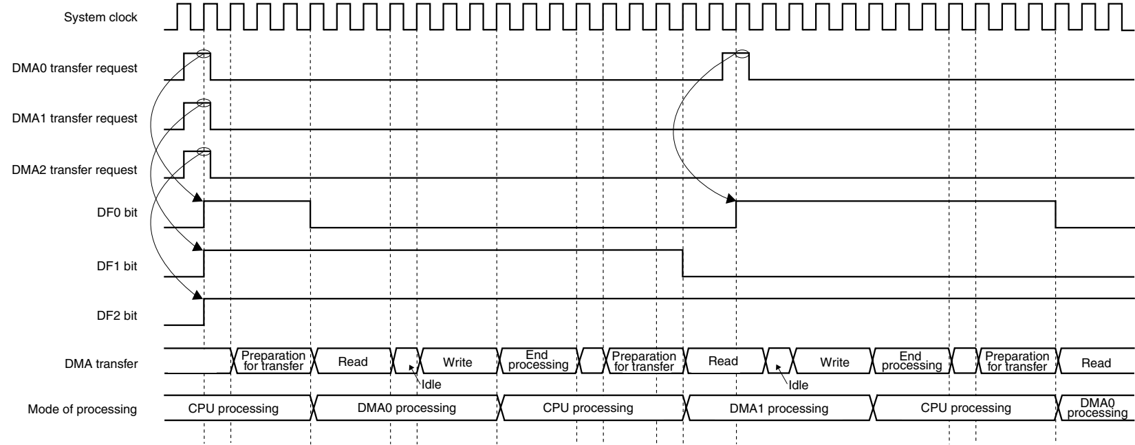
Figure 15-2. Priority of DMA (2)
