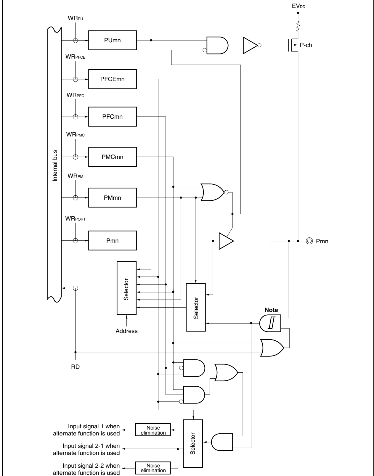
Figure 4-23. Block Diagram of Type U-7
