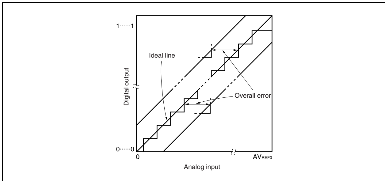
Figure 12-13. Overall Error
