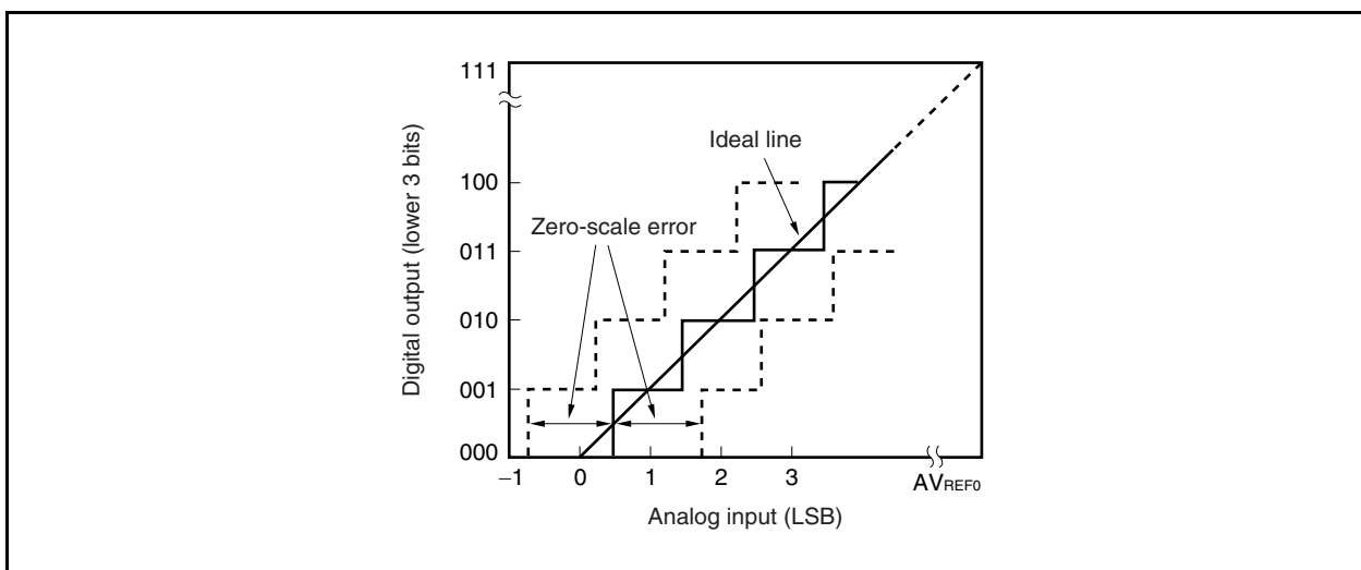
Figure 12-15. Zero-Scale Error
