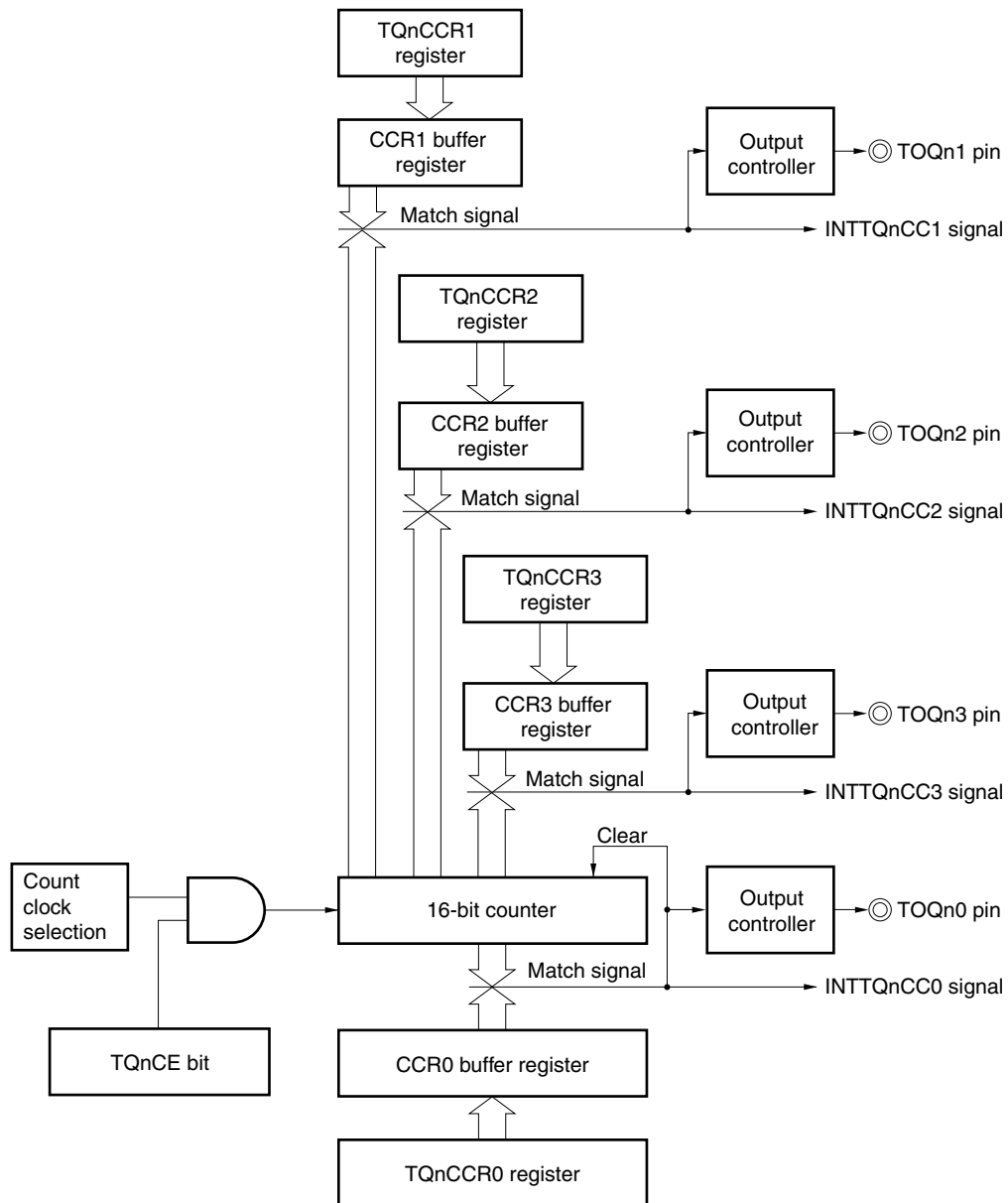
Figure 8-6. Configuration of TQnCCR1 to TQnCCR3 Registers
