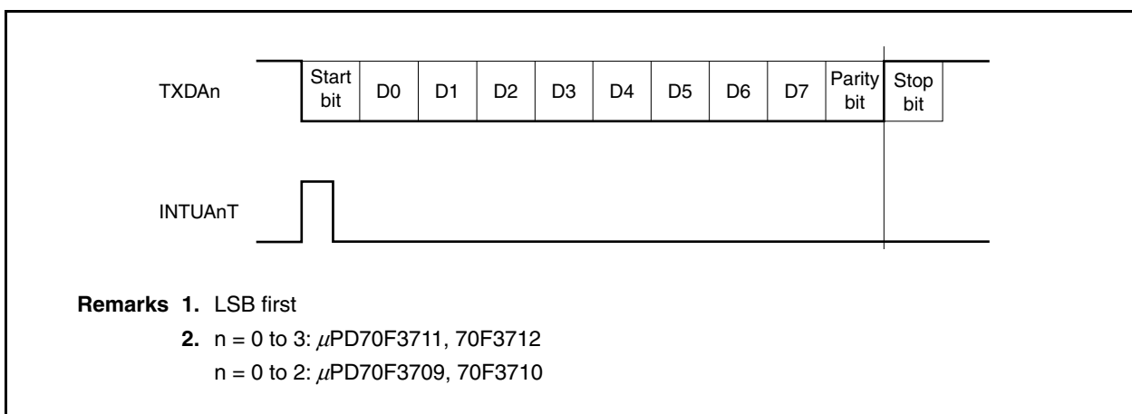
Figure 13-7. UART Transmission
