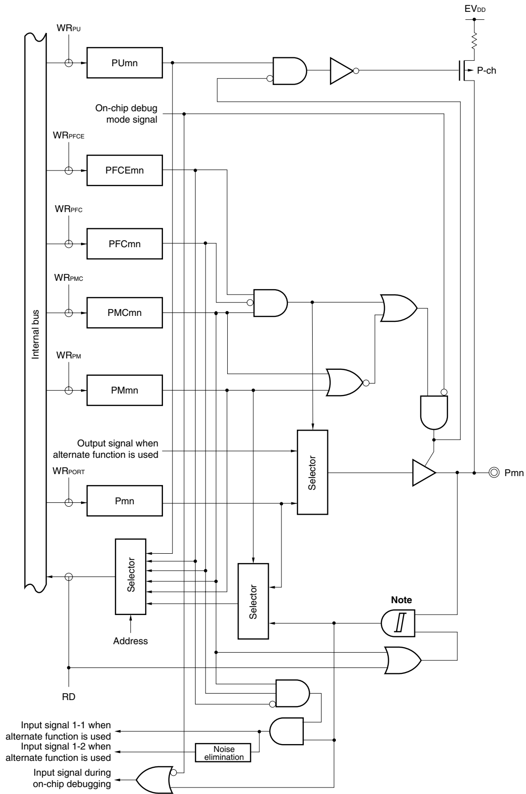
Figure 4-21. Block Diagram of Type U-5
