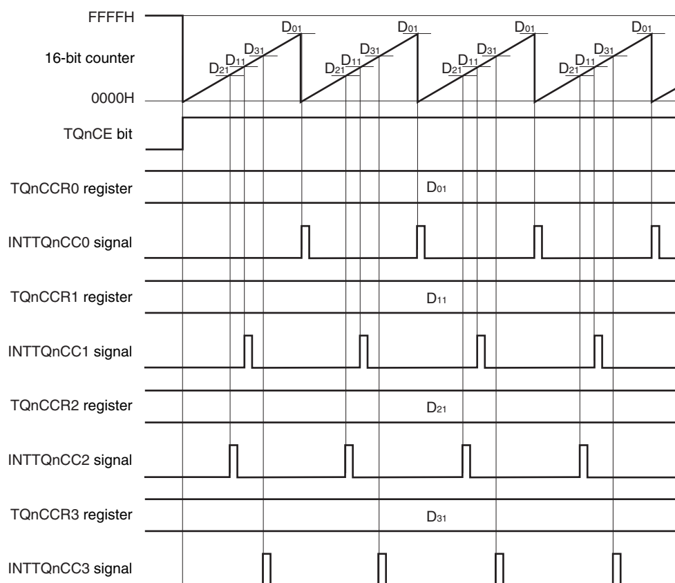
Figure 8-14. Timing Chart When D_{01} \geq D_{k1}
