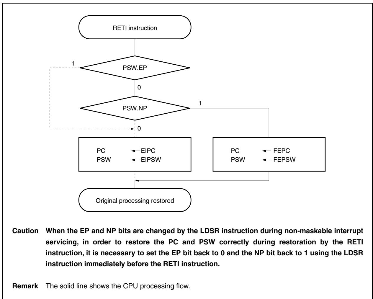
Figure 16-3. RETI Instruction Processing
