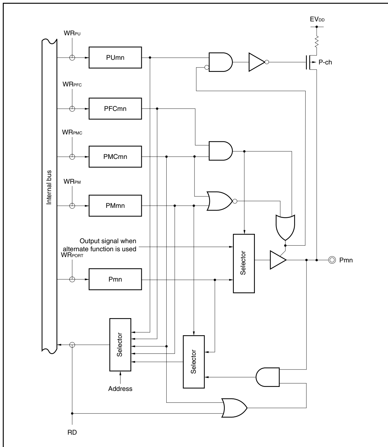
Figure 4-13. Block Diagram of Type G-3
