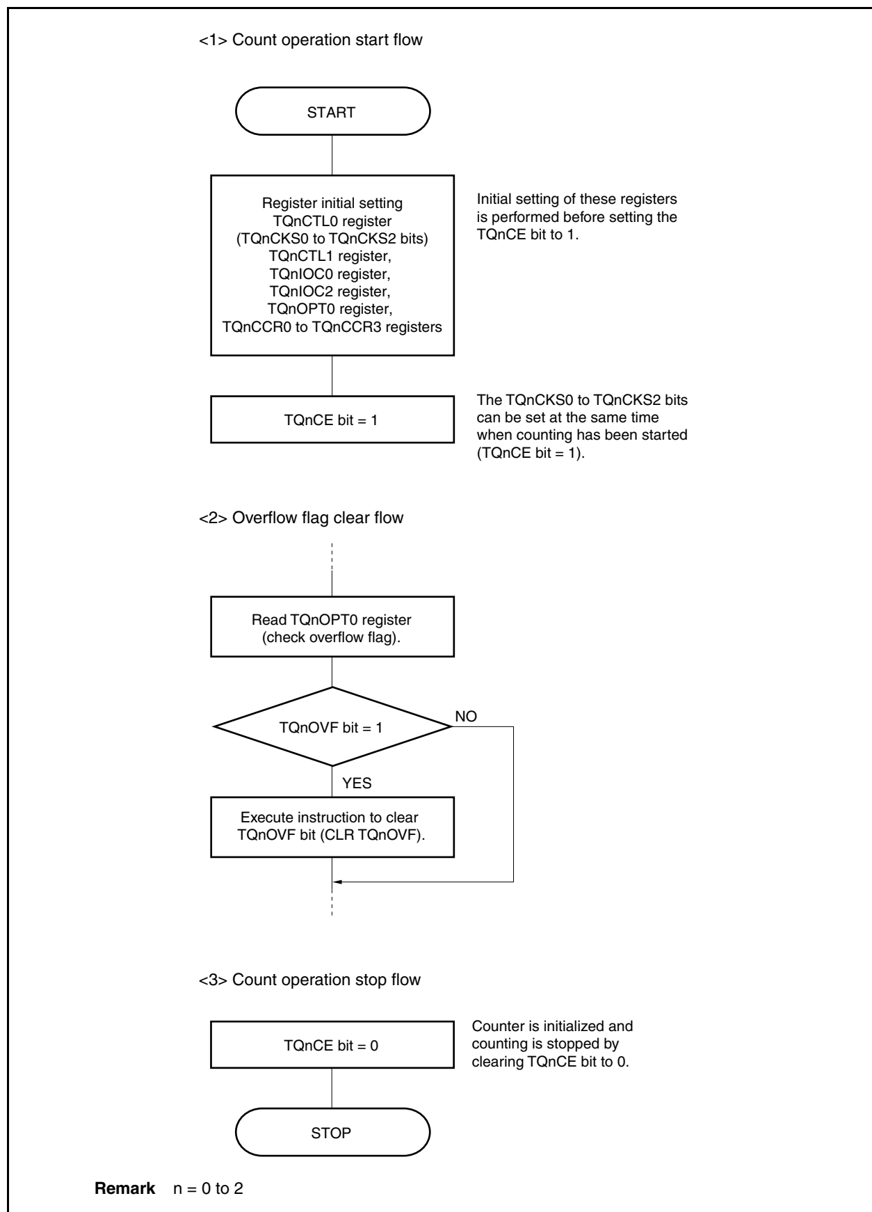
Figure 8-32. Software Processing Flow in Free-Running Timer Mode (Compare Function) (2/2)
