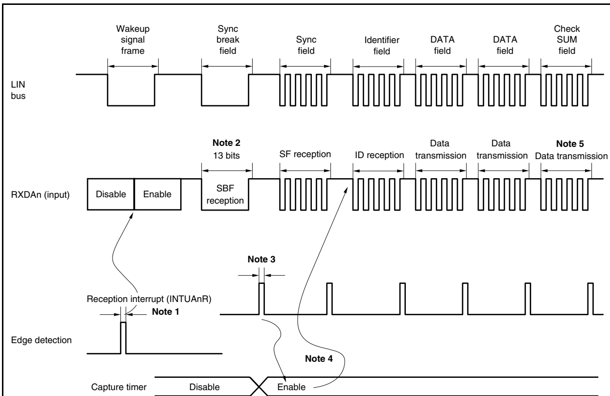
Figure 13-4. LIN Reception Manipulation Outline
