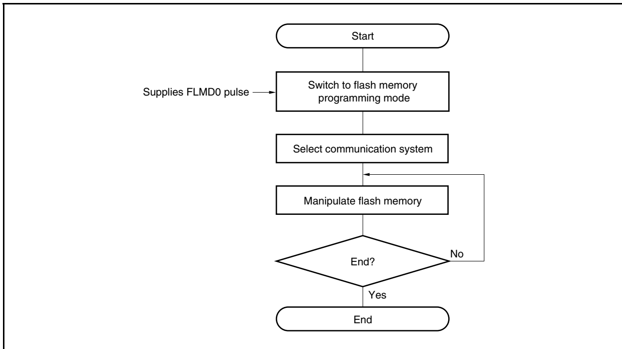
Figure 24-7. Procedure for Manipulating Flash Memory
