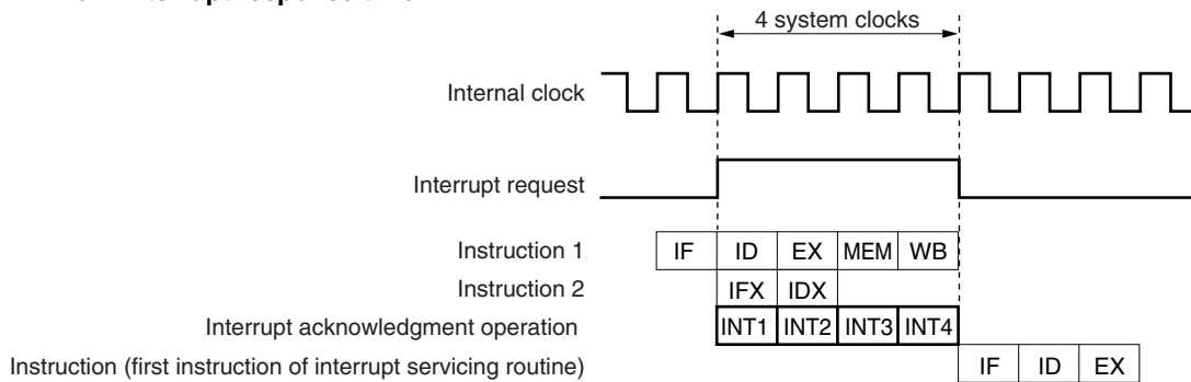
Figure 16-15. Pipeline Operation at Interrupt Request Signal Acknowledgment (Outline)
