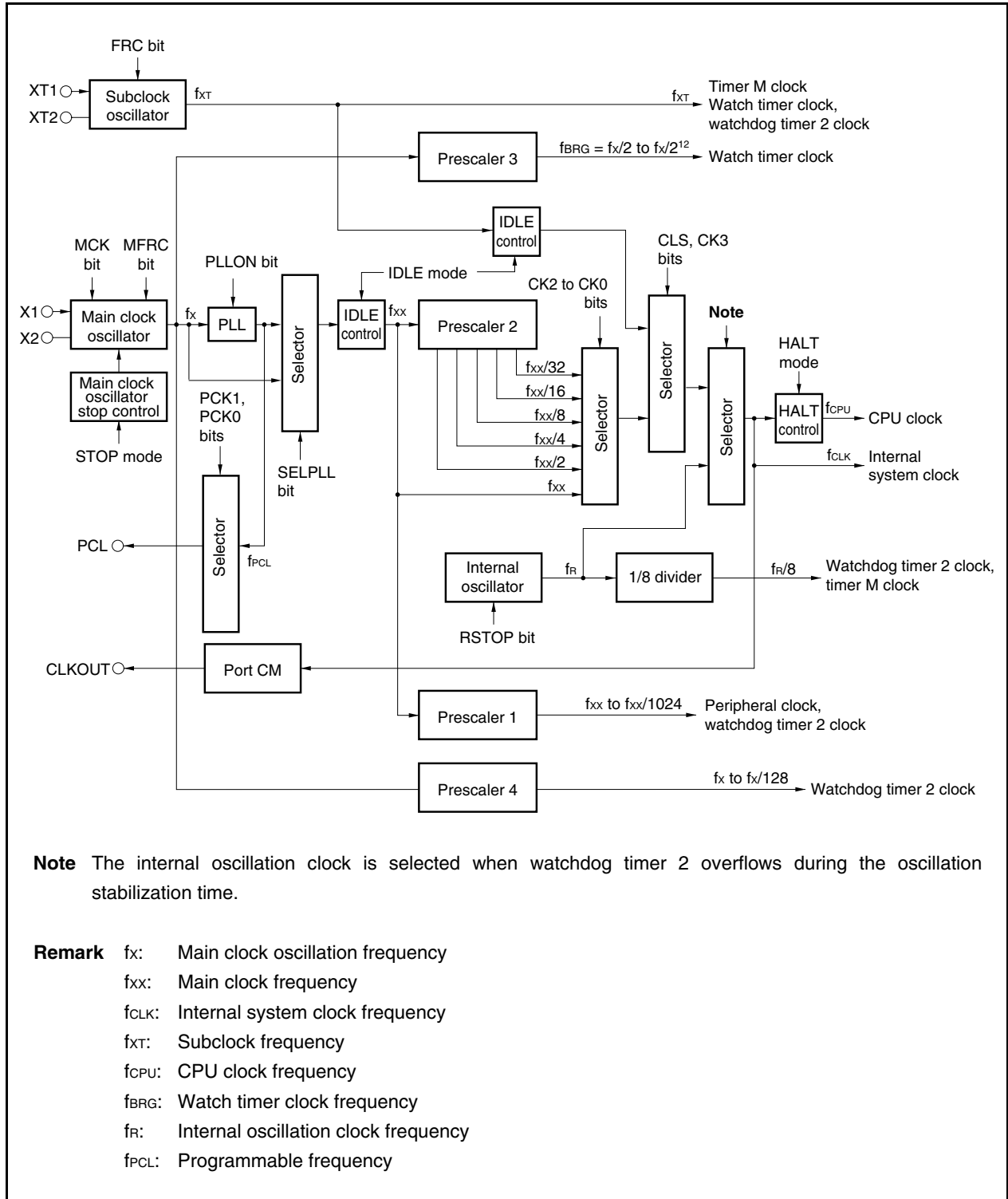
Figure 6-1. Clock Generator
