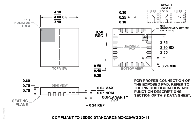
Figure 54. 20-Lead, Lead Frame Chip Scale Package [LFCSP] 4 mm x 4 mm Body and 0.75 mm Package Height (CP-20-8) Dimensions shown in millimeters
