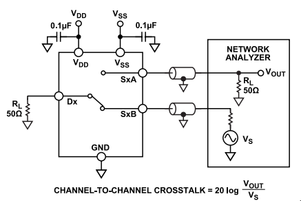
Figure 39. Channel-to-Channel Crosstalk
