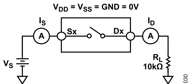
Figure 31. Switch Unpowered Leakage
