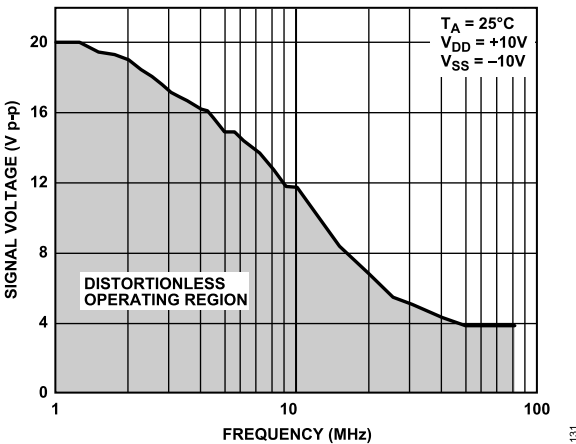
Figure 30. Large Signal Voltage Tracking vs. Frequency
