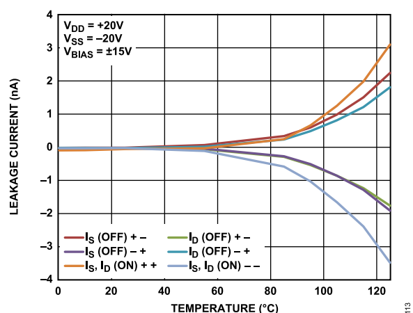
Figure 12. Leakage Current vs. Temperature, \pm 20 V Dual Supply
