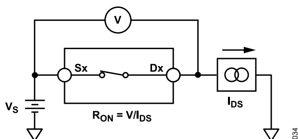
Figure 35. On Resistance
