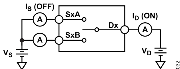
Figure 33. Off Leakage
