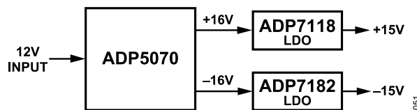
Figure 52. Bipolar Power Solution
