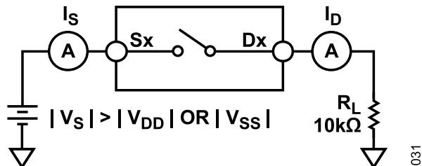
Figure 32. Switch Overvoltage Leakage
