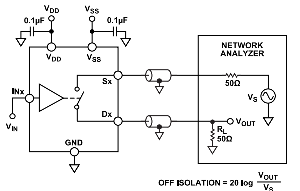
Figure 37. Off Isolation
