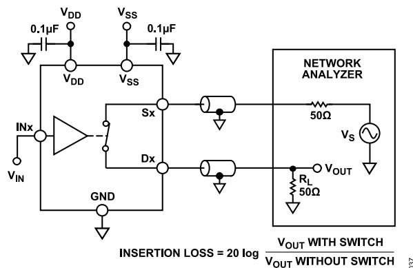
Figure 38. Bandwidth
