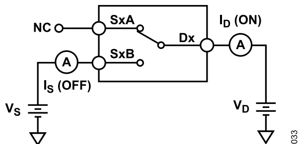
Figure 34. On Leakage
