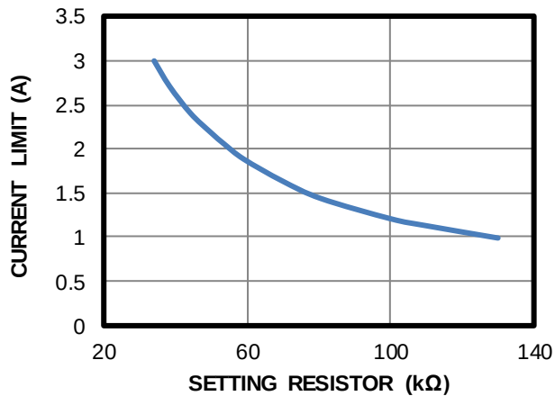
Switching Current Limit vs. Setting Resistor L = 47\mu H
