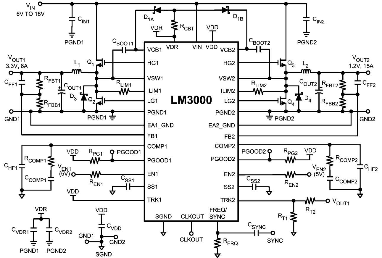
FIGURE 24. Typical Application Schematic
