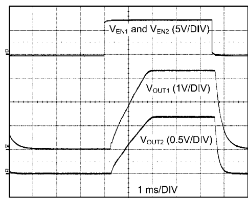
Soft-Start with Load
