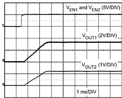
Soft-Start without Load
