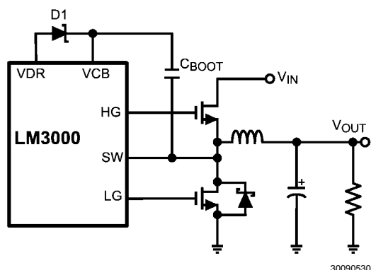
FIGURE 9. Bootstrap Circuit
