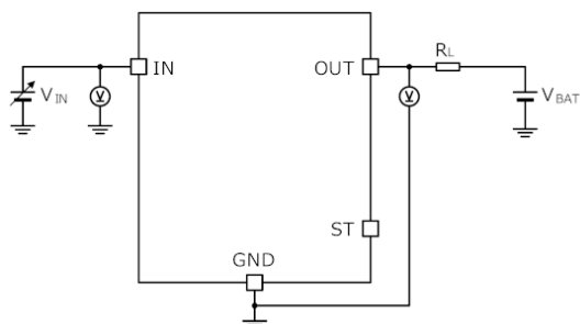
Measurement Circuit for Figure 2
