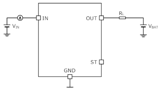
Measurement Circuit for Figure 3, Figure 4
