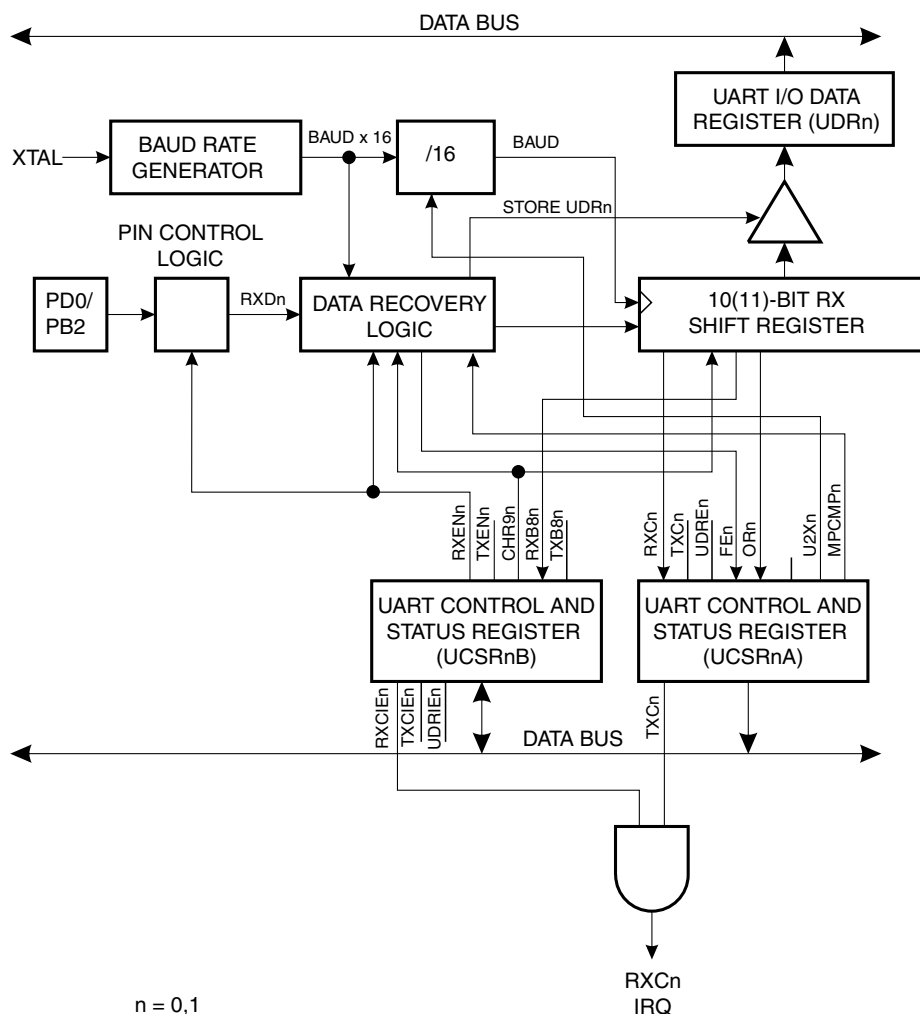
Figure 45. UART Receiver
