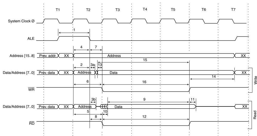
Figure 86. External Memory Timing (SRWn1 = 1, SRWn0 = 1) (1)
