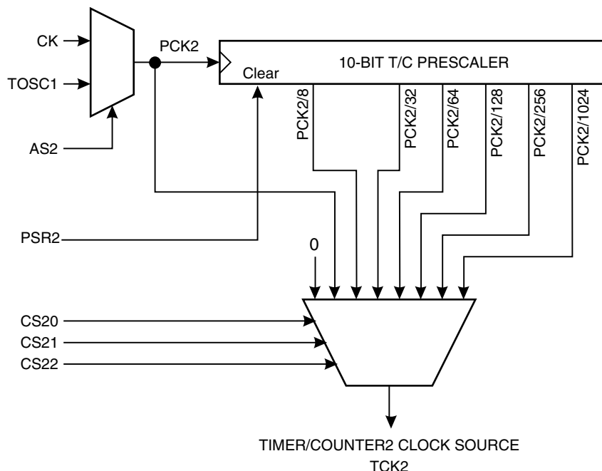
Figure 30. Timer/Counter2 Prescaler
