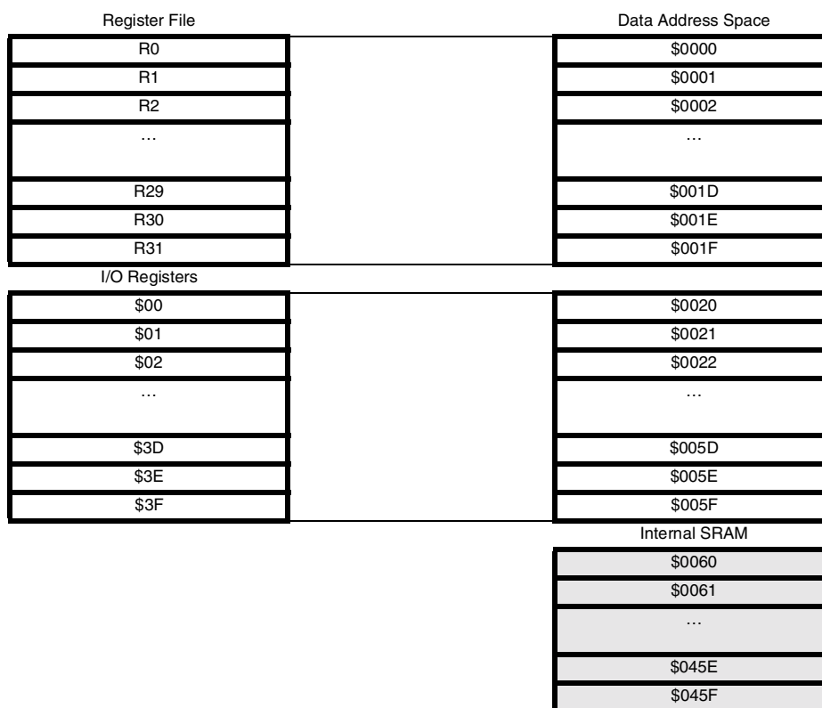
Figure 8. SRAM Organization
