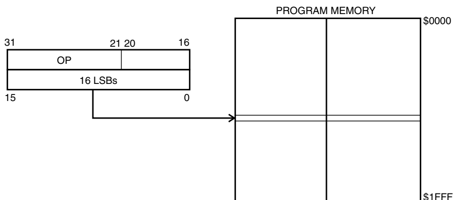
Figure 20. Direct Program Addressing
