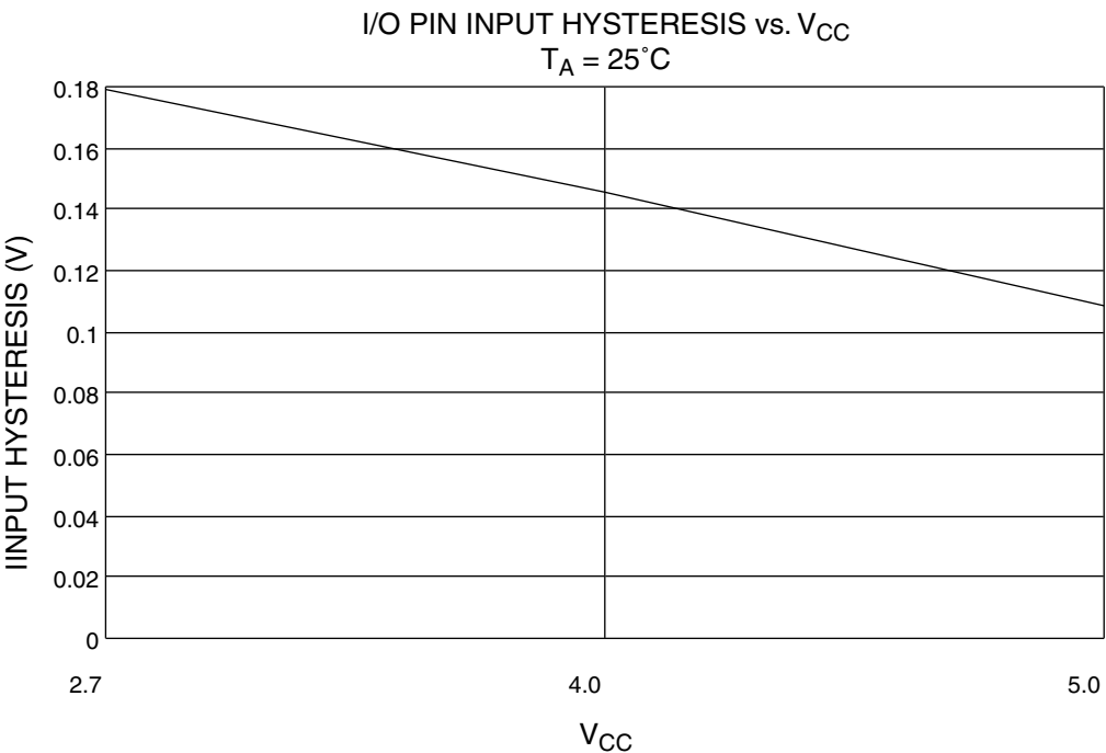
Figure 98. I/O Pin Input Hysteresis vs. V_{CC}
