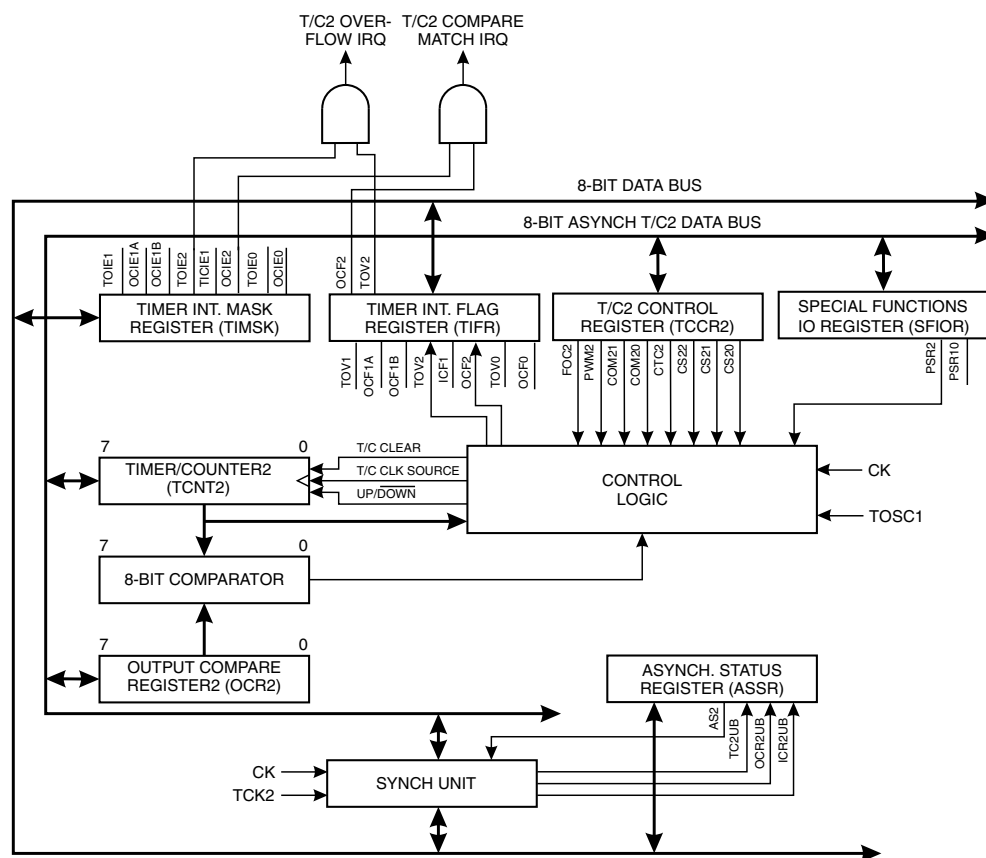
Figure 32. Timer/Counter2 Block Diagram
