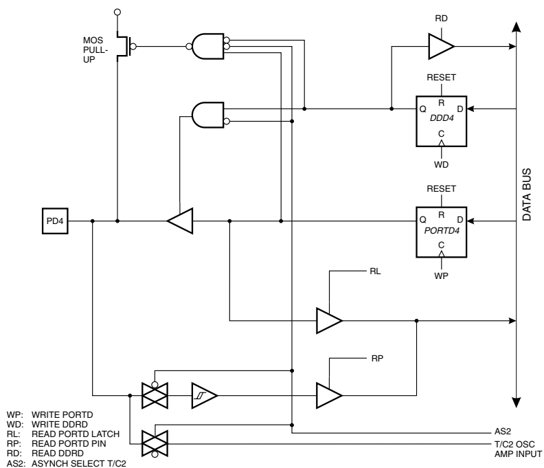
Figure 67. Port D Schematic Diagram (Pin PD4)
