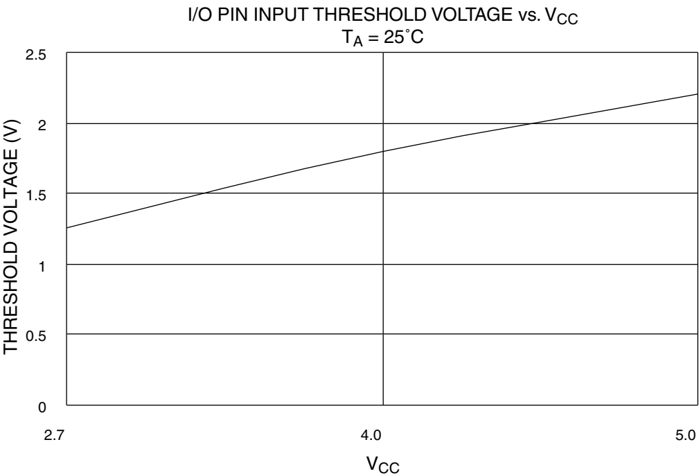
Figure 97. I/O Pin Input Threshold vs. V_{CC}
