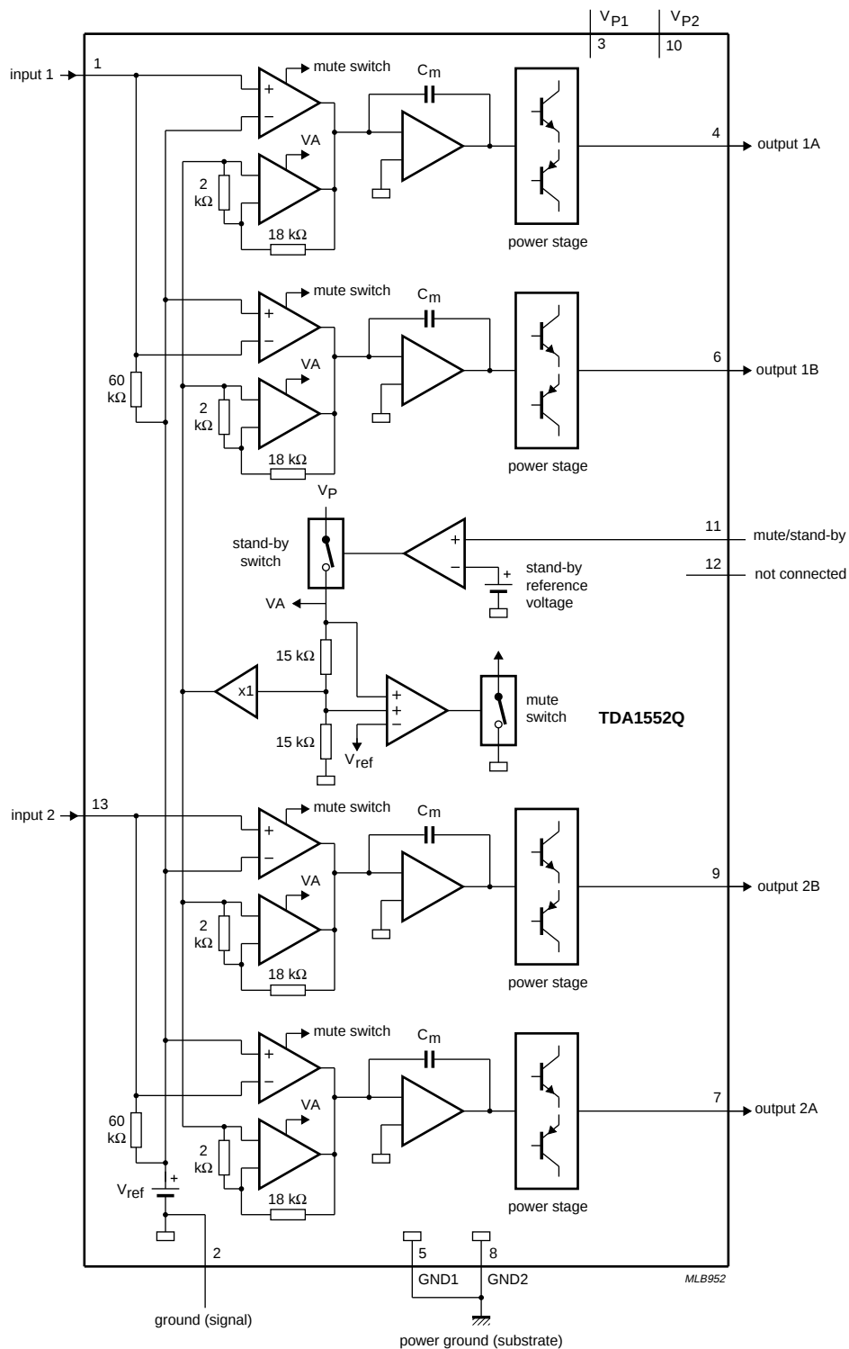
Fig.1 Block diagram.
