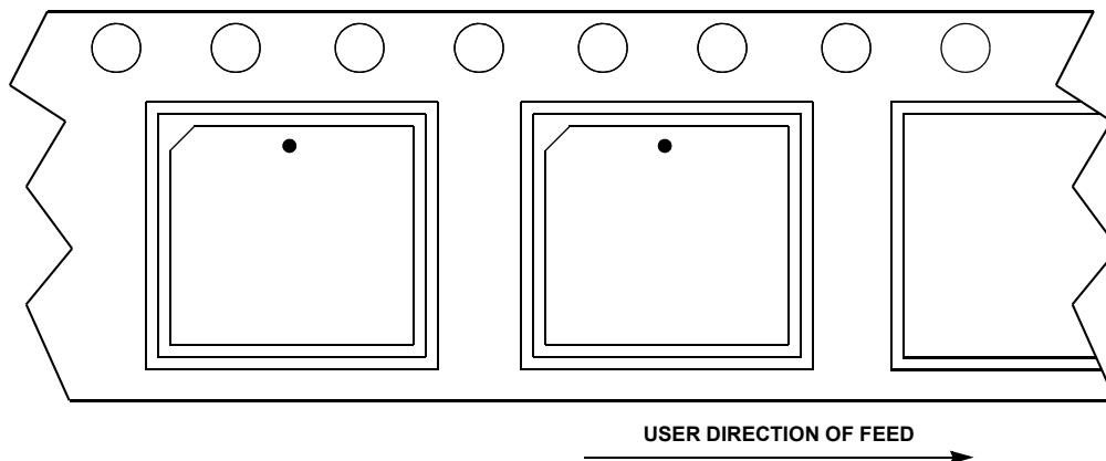
FIGURE 5C. PLCC
