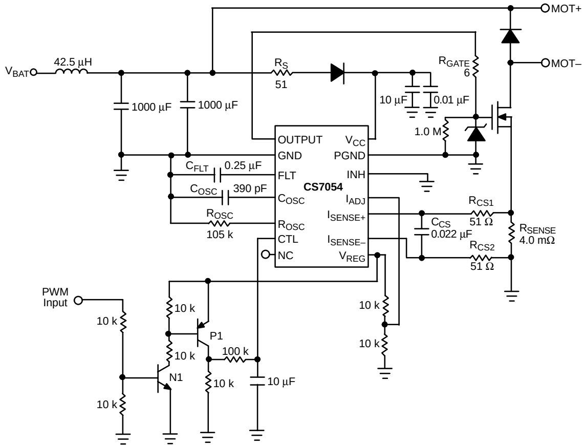
Figure 1. Application Diagram
