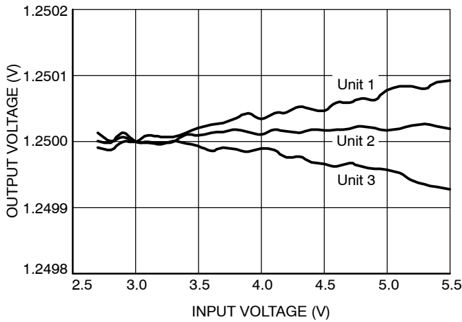
Figure 4. Line Regulation
