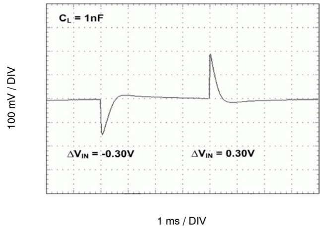
Figure 9. Line Transient Response with Capacitive Load
