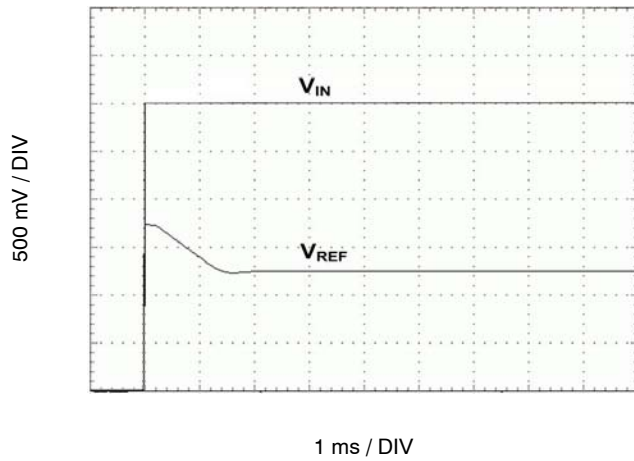
Figure 14. Turn-On Time
