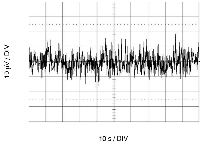
Figure 15. Output Noise
