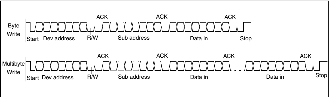
Figure 16. I 2 C write operations
