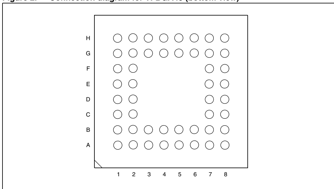
Figure 2. Connection diagram for TFBGA48 (bottom view)
