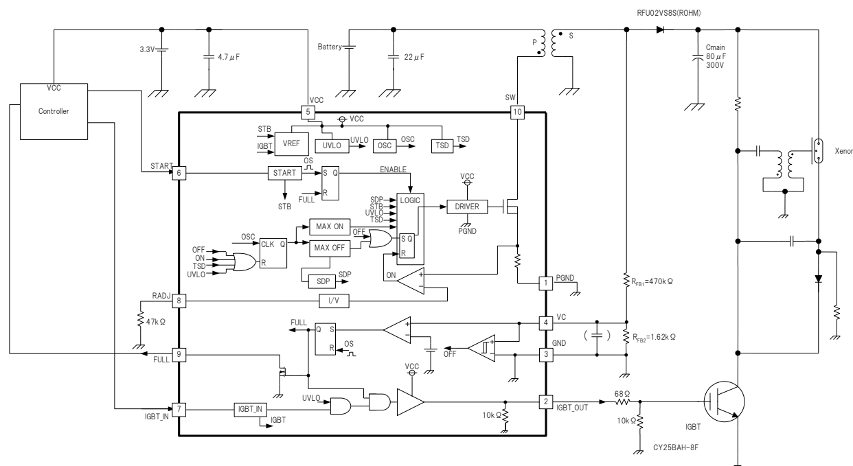
Fig.1 Application circuit
