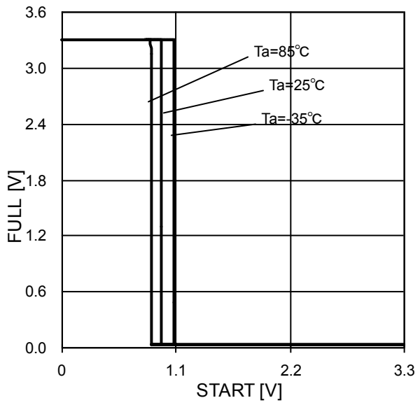
Fig.15 Start Threshold Voltage
