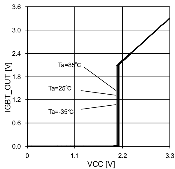
Fig.13 VCC UVLO Check (IGBT) (Sweep Down)
