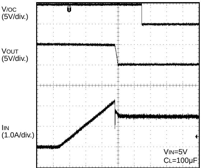
TIME(4ms/div.) Figure 35. Over-Current Response Ramped Load
