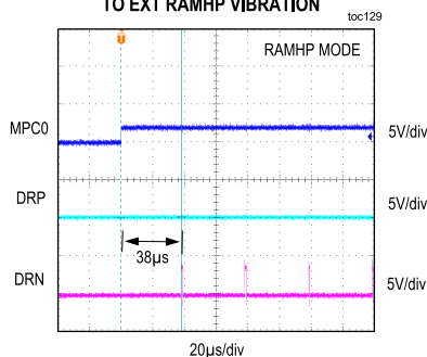
HAPTIC DRIVER TIME FROM MPC0 ASSERTION TO EXT RAMHP VIBRATION
