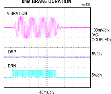
HAPTIC DRIVER 200ms ERM DRIVE 0ms BRAKE DURATION
