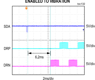
HAPTIC DRIVER TIME FROM HptDrvClkEn ENABLED TO VIBRATION
