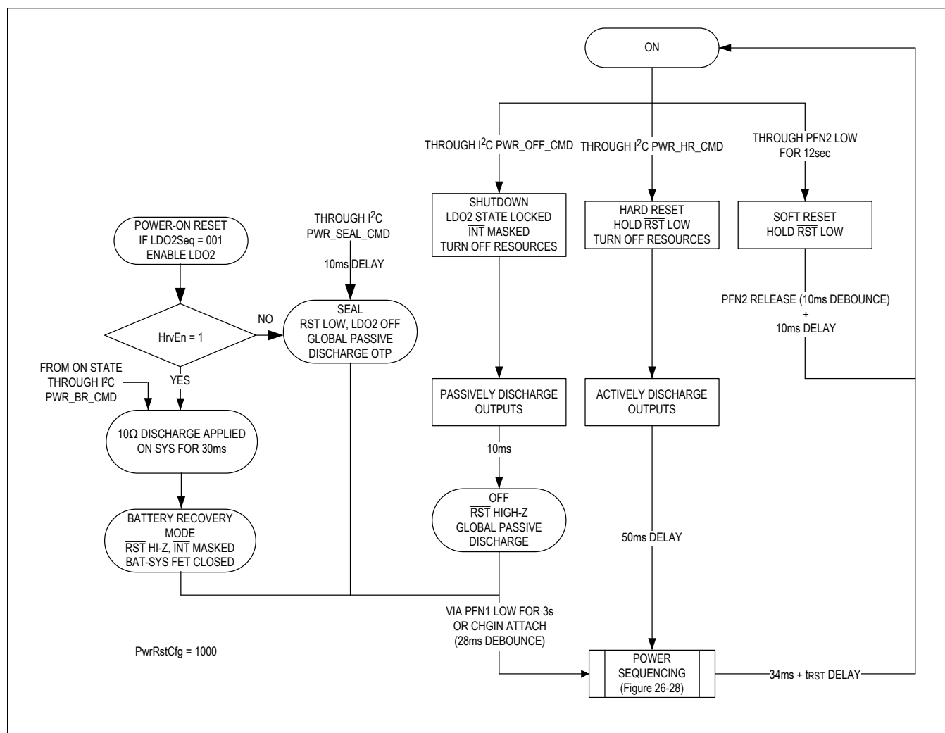
Figure 20. PwrRstCfg 1000
