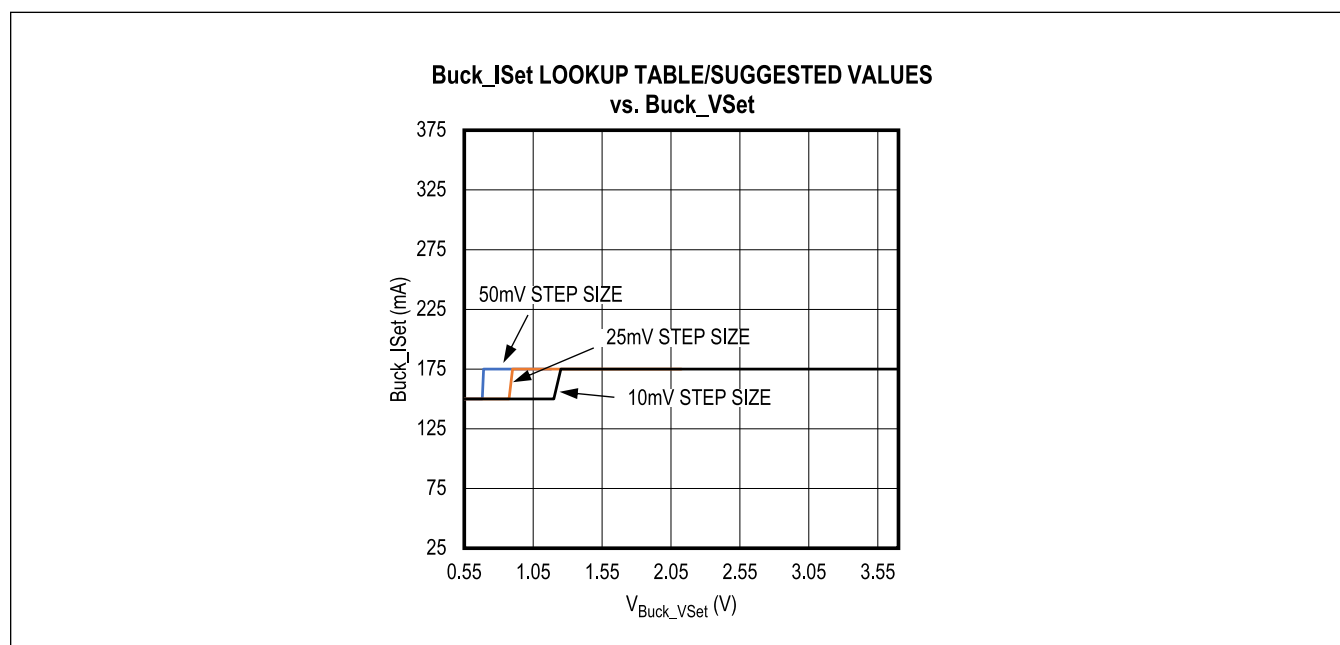
Figure 14. Optimal Peak Current Setting vs. Output Voltage
