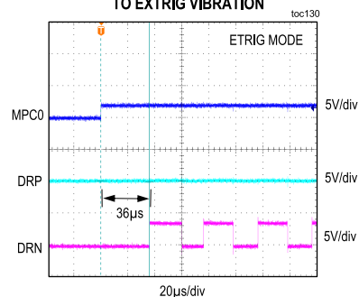
HAPTIC DRIVER TIME FROM MPC0 ASSERTION TO EXTRIG VIBRATION
