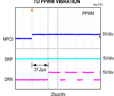
HAPTIC DRIVER TIME FROM MPC0 ASSERTION TO PPWM VIBRATION
