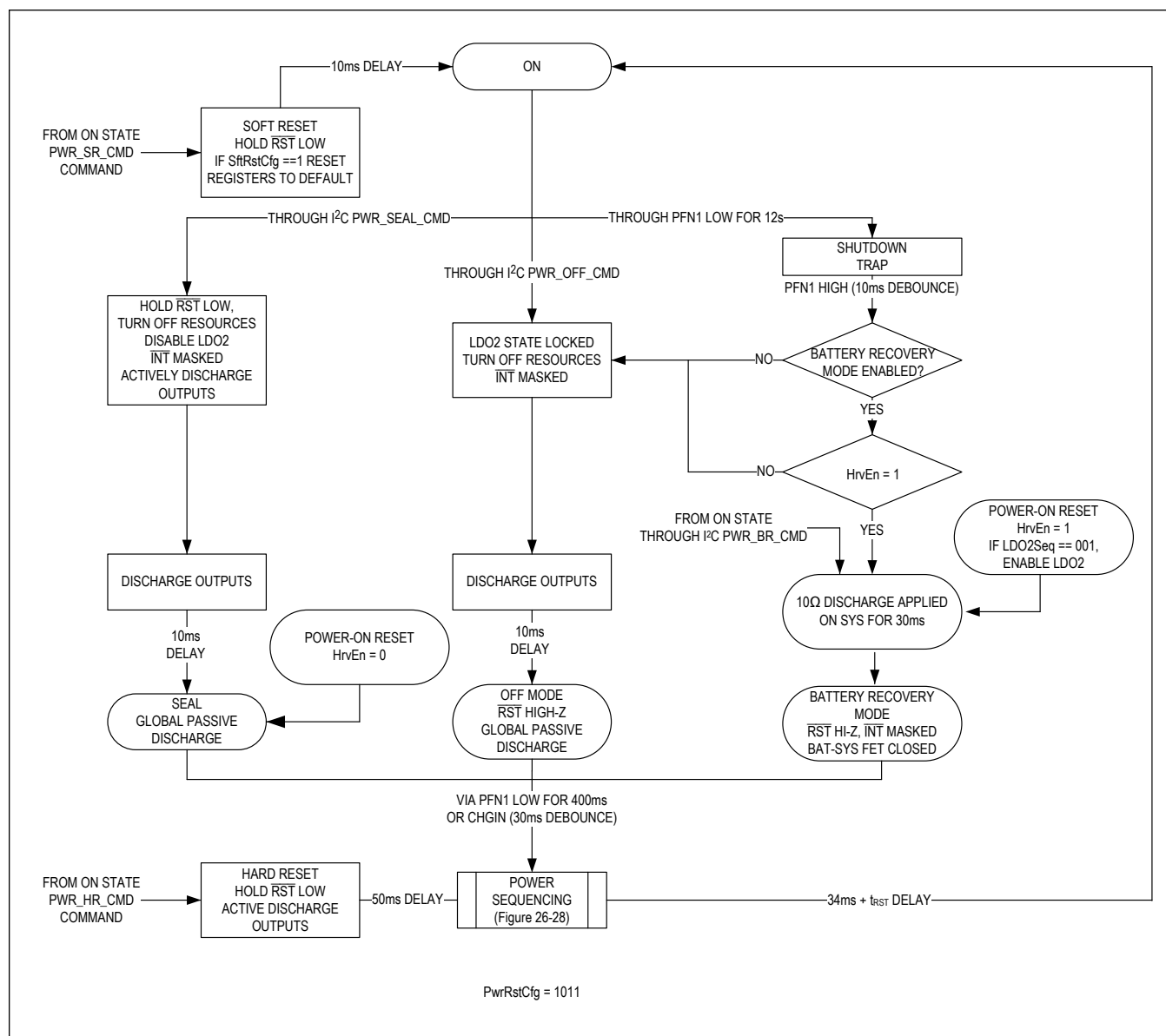
Figure 22. PwrRstCfg 1011
