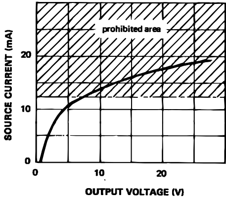
ALARM OUTPUT CURRENT SOURCE (normal operation).
