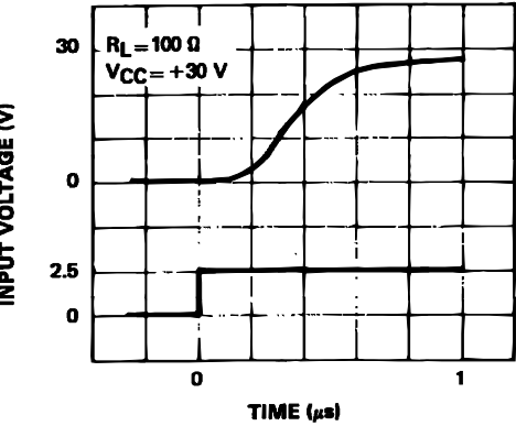
RESPONSE TIME.
