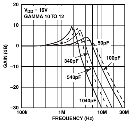
TPC 7. Frequency Response vs. Capacitive Loading
