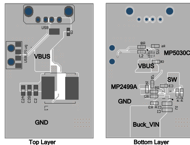
Figure 7: Recommended Layout
