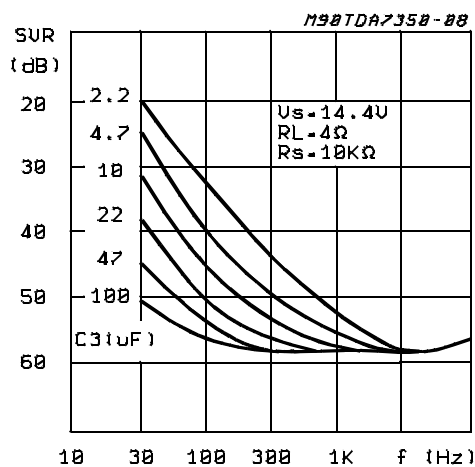
Figure 18: SVR vs. Frequency & C_{SVR} ; (Bridge)
