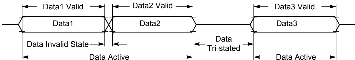
Figure 3-5 Signal States
