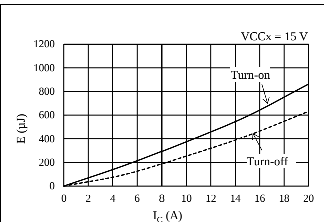
Figure 15-35. Low-side Switching Loss ( T_J = 25^\circ\text{C} )
