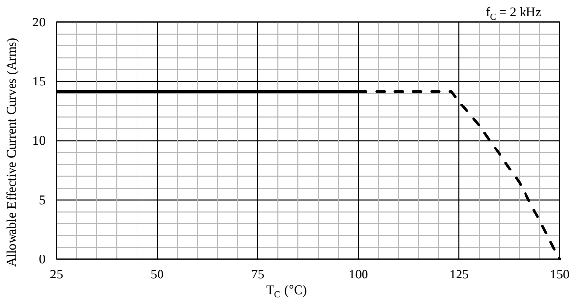
Figure 15-44. Allowable Effective Current ( f_C = 2 \text{ kHz} ): SCM1274MF
