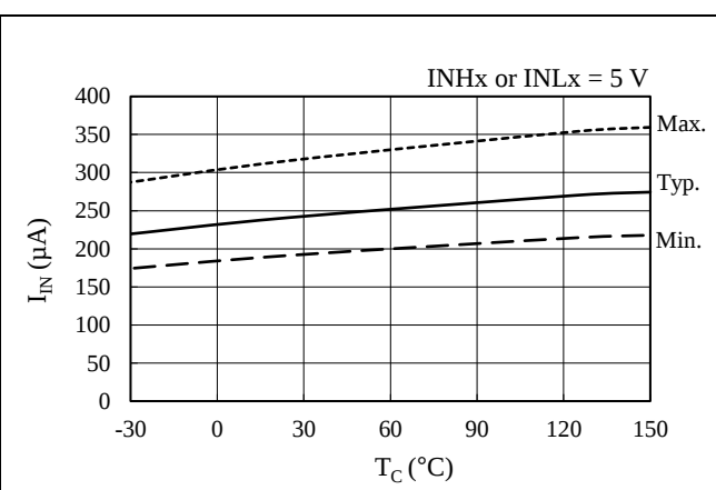
Figure 15-12. Input Current at High Level ( I_{INHx} or I_{LINx} ), I_{IN} vs. T_C
