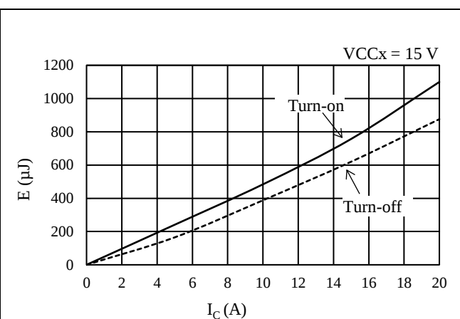
Figure 15-37. Low-side Switching Loss ( T_J = 125^\circ\text{C} )
