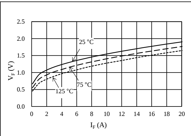
Figure 15-27. Freewheeling Diode V_F vs. I_F
