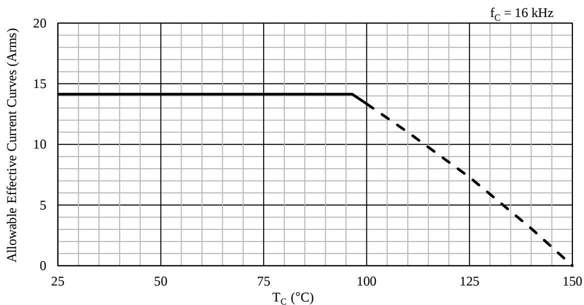
Figure 15-45. Allowable Effective Current ( f_C = 16 \text{ kHz} ): SCM1274MF
