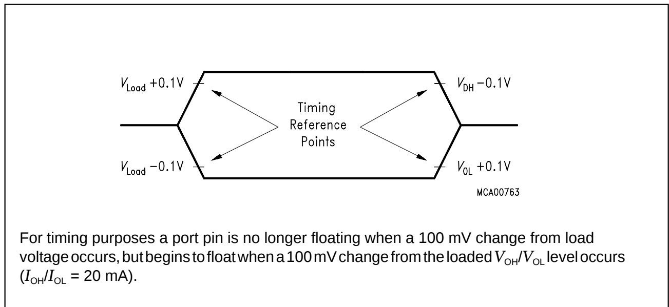
Figure 10 Float Waveforms
