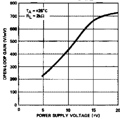
OPEN-LOOP GAIN vs SUPPLY VOLTAGE
