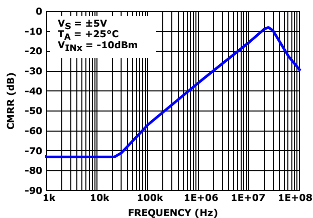
FIGURE 23. CMRR
