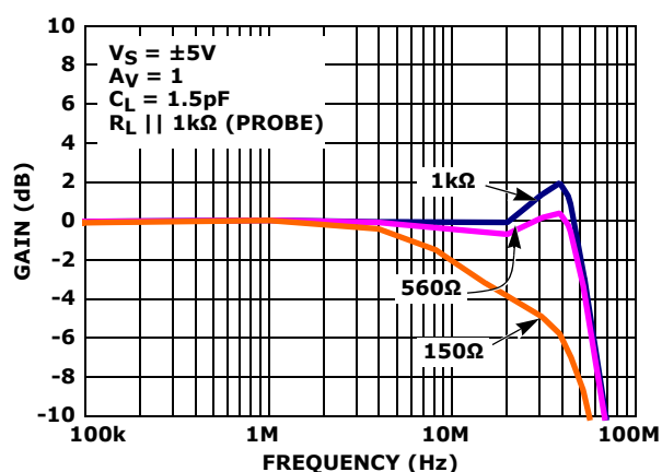
FIGURE 18. FREQUENCY RESPONSE FOR VARIOUS R_L
