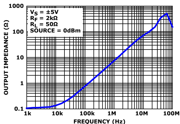
FIGURE 20. CLOSED LOOP OUTPUT IMPEDANCE
