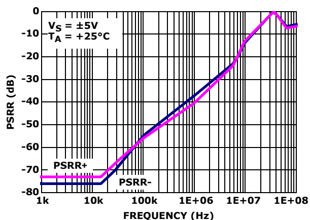
FIGURE 24. PSRR
