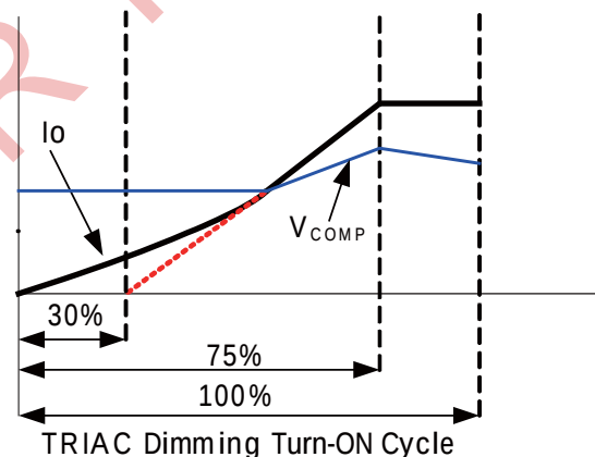
Figure 13: Dimming Curve
