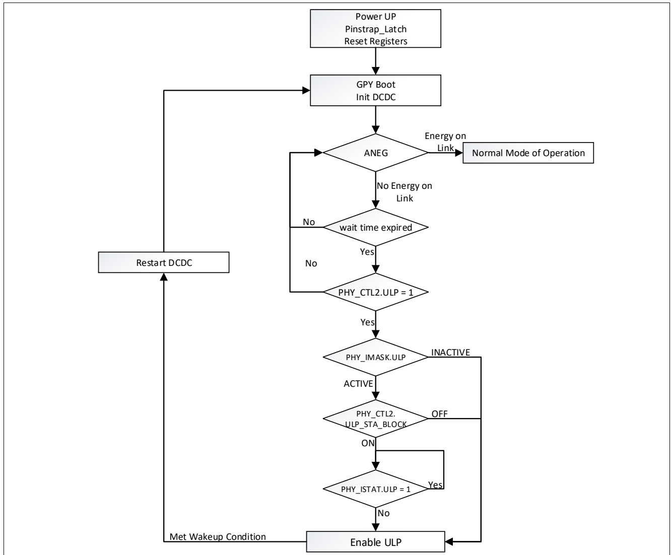
Figure 15 ULP Sequence
