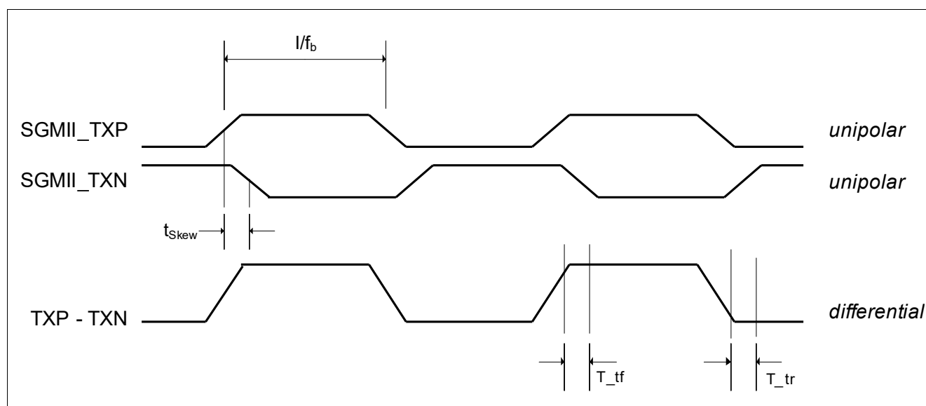
Figure 22 Transmit Timing Diagram of the SGMII (shows alternating data sequence)
