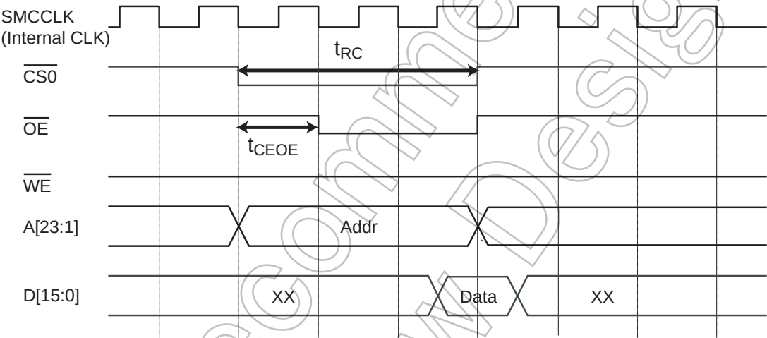
Figure 10-2 Asynchronous Read
