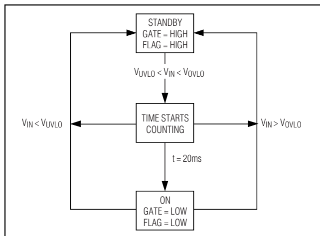
Figure 2. State Machine
