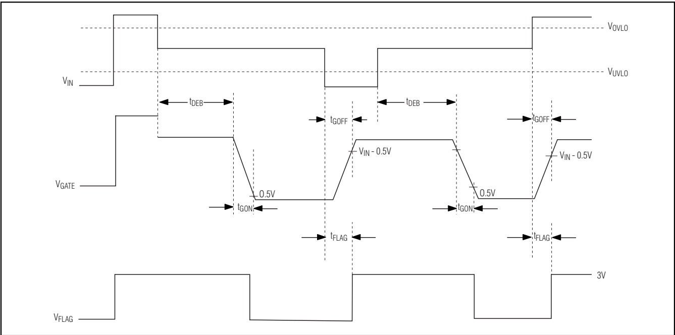
Figure 1. Timing Diagram
