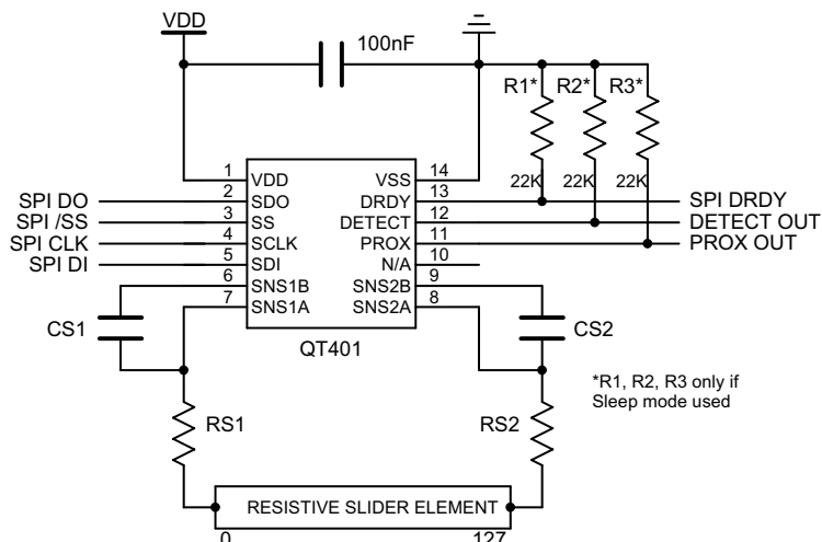
Figure 1-1 QT401 Wiring Diagram
