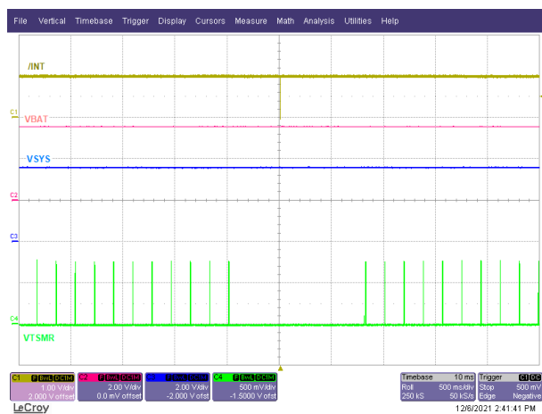
Figure 9-18. Wake1 Interrupt without VIN
