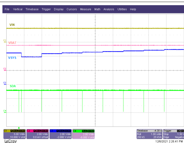
Figure 9-13. SYS Regulation Sweep
