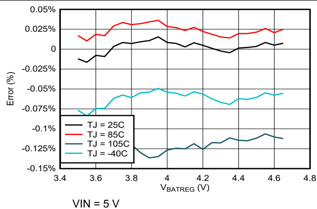
Figure 7-1. Battery Regulation Voltage Accuracy vs VBATREG Setting
