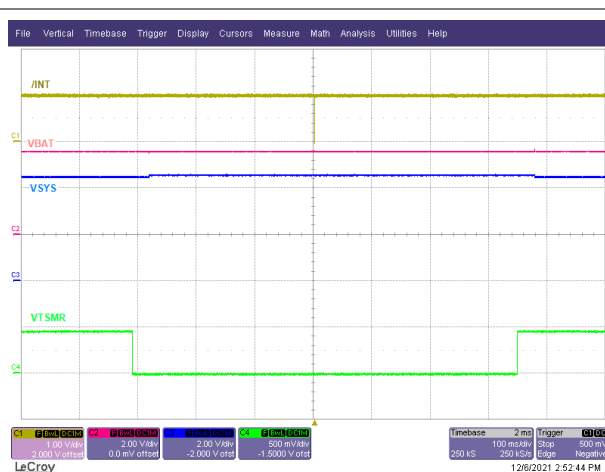
Figure 9-15. Wake1 Interrupt with VIN Present
