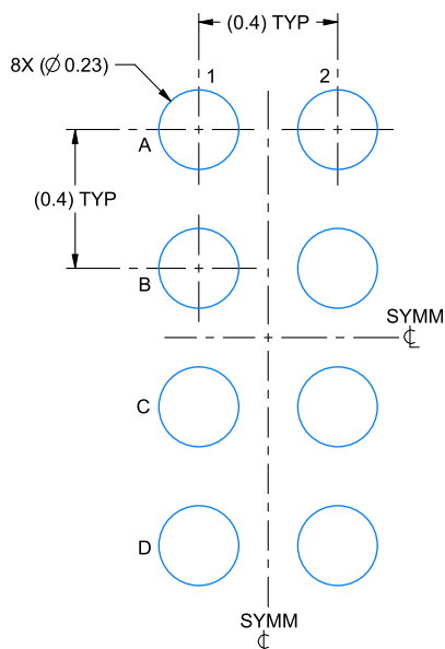
LAND PATTERN EXAMPLE EXPOSED METAL SHOWN SCALE: 50X
